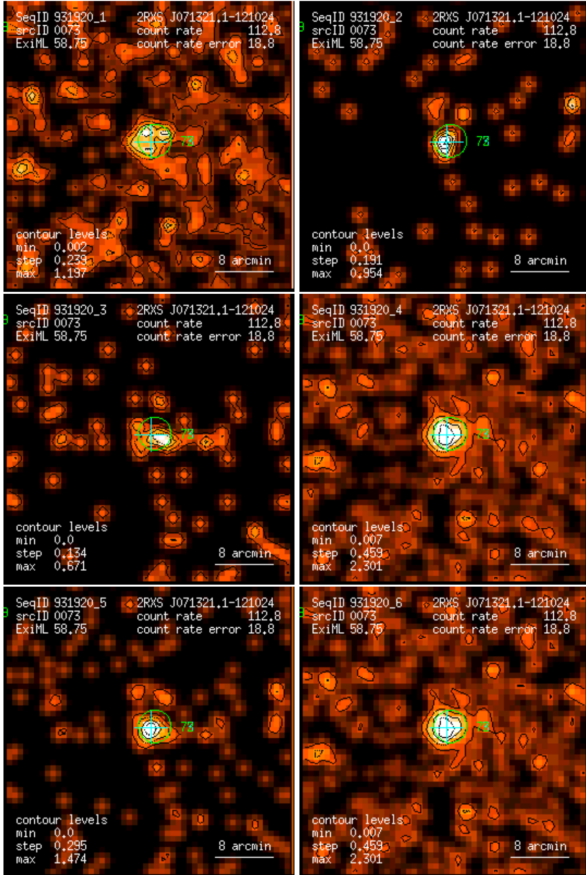
Figure 73: RASS 931920: detection 0073: band rate images, Gaussian filter: (1) PSPC channels 11 – 41, (2) 52 – 90, (3) 91 – 201, (4) 11 – 235, (5) 52 – 201, (6) 11 – 201. Broad band rates in counts/ks. Band rate contour levels in counts/ks/arcmin 2 .
