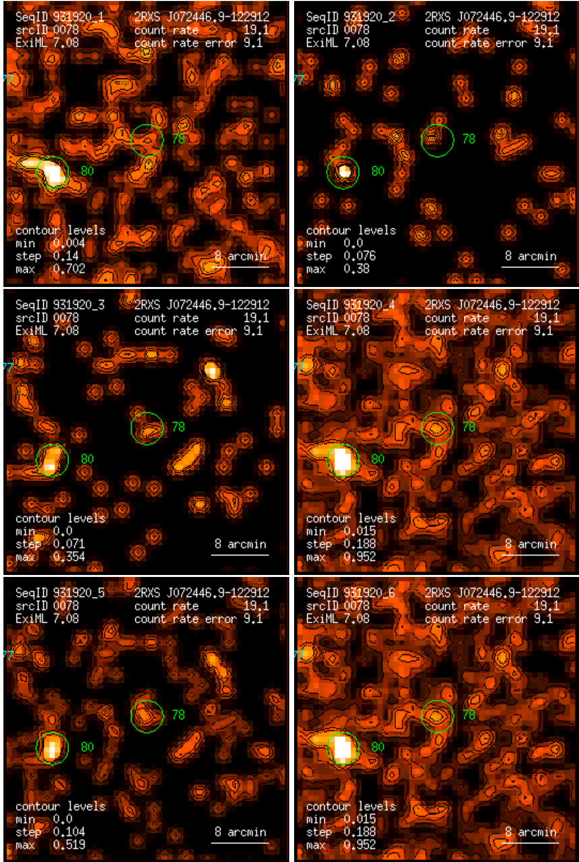
Figure 78: RASS 931920: detection 0078: band rate images, Gaussian filter: (1) PSPC channels 11 – 41, (2) 52 – 90, (3) 91 – 201, (4) 11 – 235, (5) 52 – 201, (6) 11 – 201. Broad band rates in counts/ks. Band rate contour levels in counts/ks/arcmin 2 .
