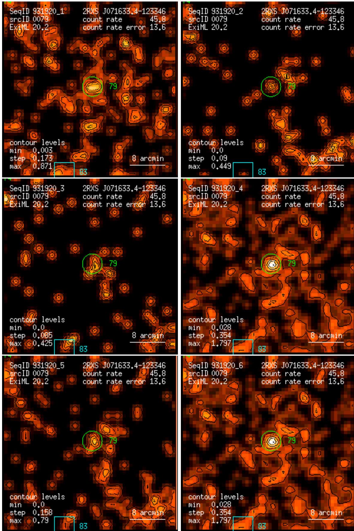
Figure 79: RASS 931920: detection 0079: band rate images, Gaussian filter: (1) PSPC channels 11 – 41, (2) 52 – 90, (3) 91 – 201, (4) 11 – 235, (5) 52 – 201, (6) 11 – 201. Broad band rates in counts/ks. Band rate contour levels in counts/ks/arcmin 2 .
