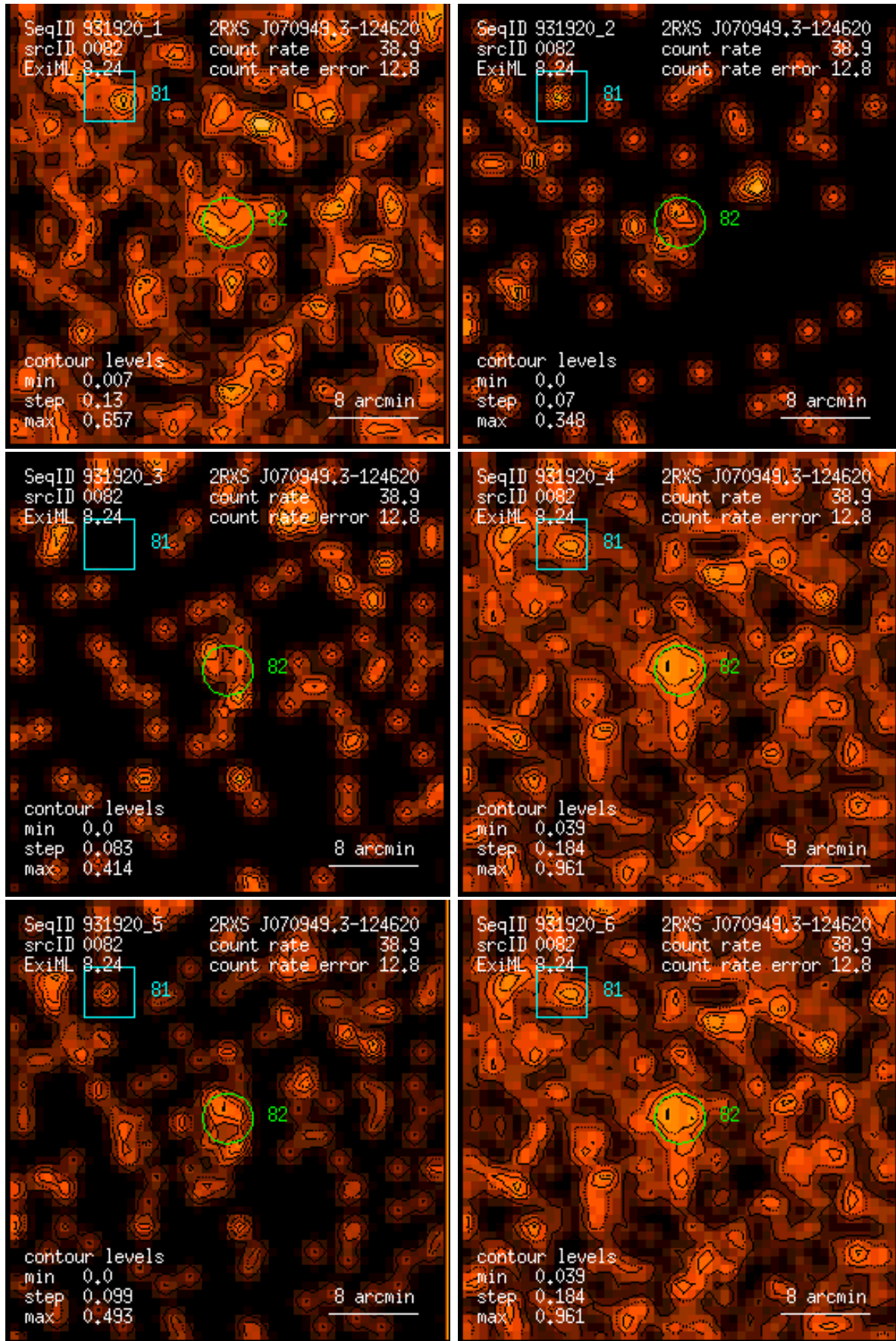
Figure 82: RASS 931920: detection 0082: band rate images, Gaussian filter: (1) PSPC channels 11 – 41, (2) 52 – 90, (3) 91 – 201, (4) 11 – 235, (5) 52 – 201, (6) 11 – 201. Broad band rates in counts/ks. Band rate contour levels in counts/ks/arcmin 2 .
