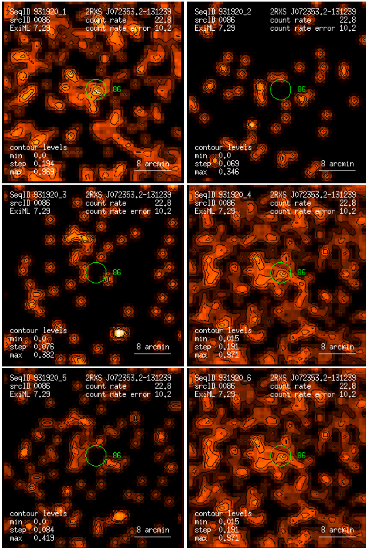
Figure 86: RASS 931920: detection 0086: band rate images, Gaussian filter: (1) PSPC channels 11 – 41, (2) 52 – 90, (3) 91 – 201, (4) 11 – 235, (5) 52 – 201, (6) 11 – 201. Broad band rates in counts/ks. Band rate contour levels in counts/ks/arcmin 2 .
