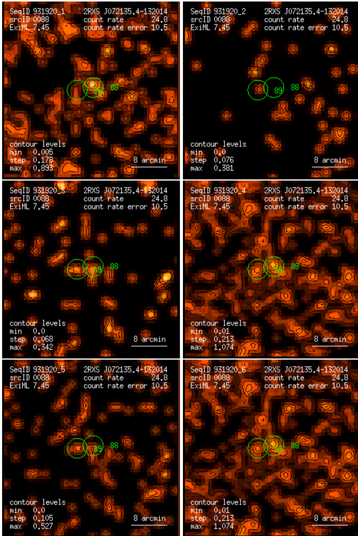
Figure 88: RASS 931920: detection 0088: band rate images, Gaussian filter: (1) PSPC channels 11 – 41, (2) 52 – 90, (3) 91 – 201, (4) 11 – 235, (5) 52 – 201, (6) 11 – 201. Broad band rates in counts/ks. Band rate contour levels in counts/ks/arcmin 2 .
