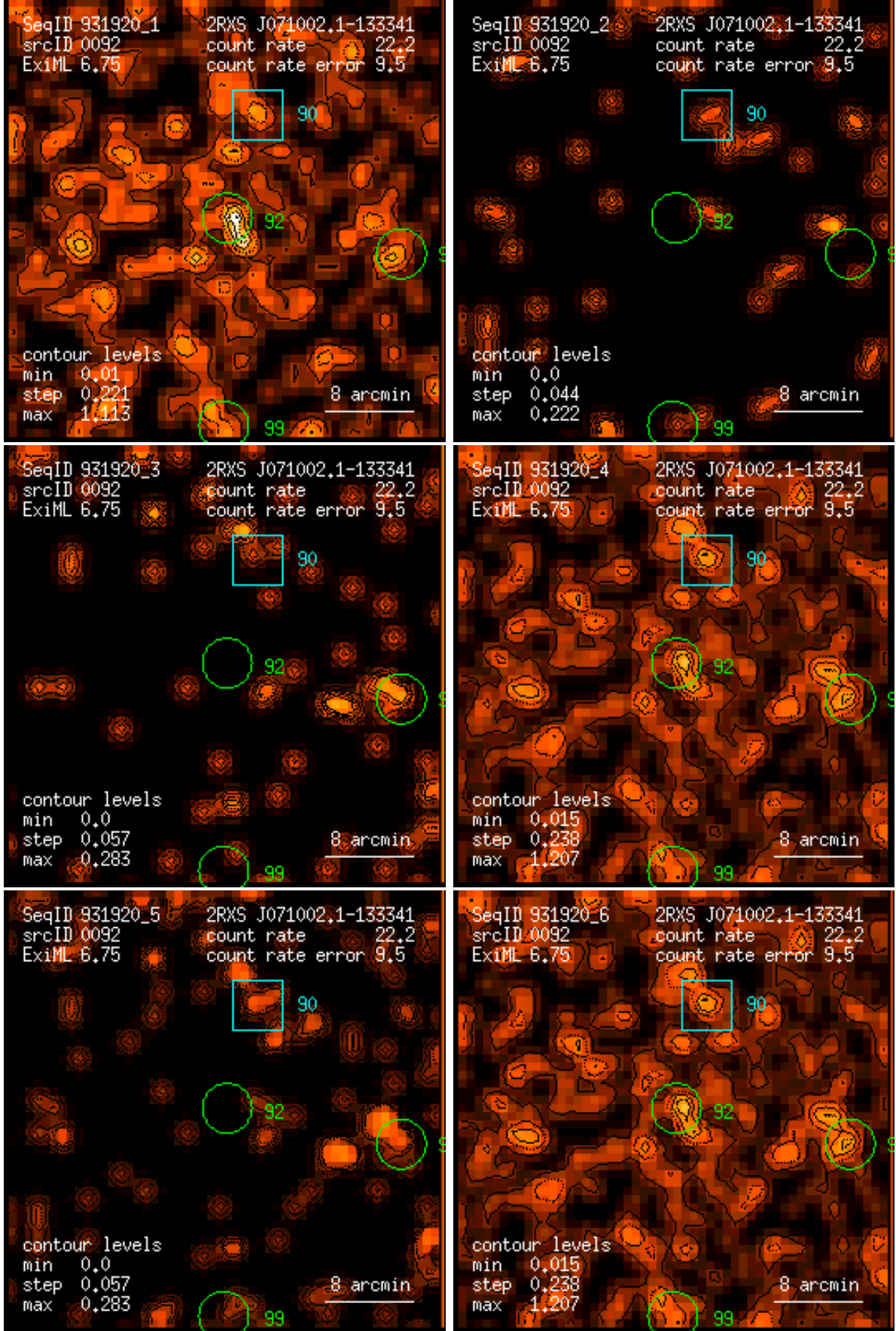
Figure 92: RASS 931920: detection 0092: band rate images, Gaussian filter: (1) PSPC channels 11 – 41, (2) 52 – 90, (3) 91 – 201, (4) 11 – 235, (5) 52 – 201, (6) 11 – 201. Broad band rates in counts/ks. Band rate contour levels in counts/ks/arcmin 2 .
