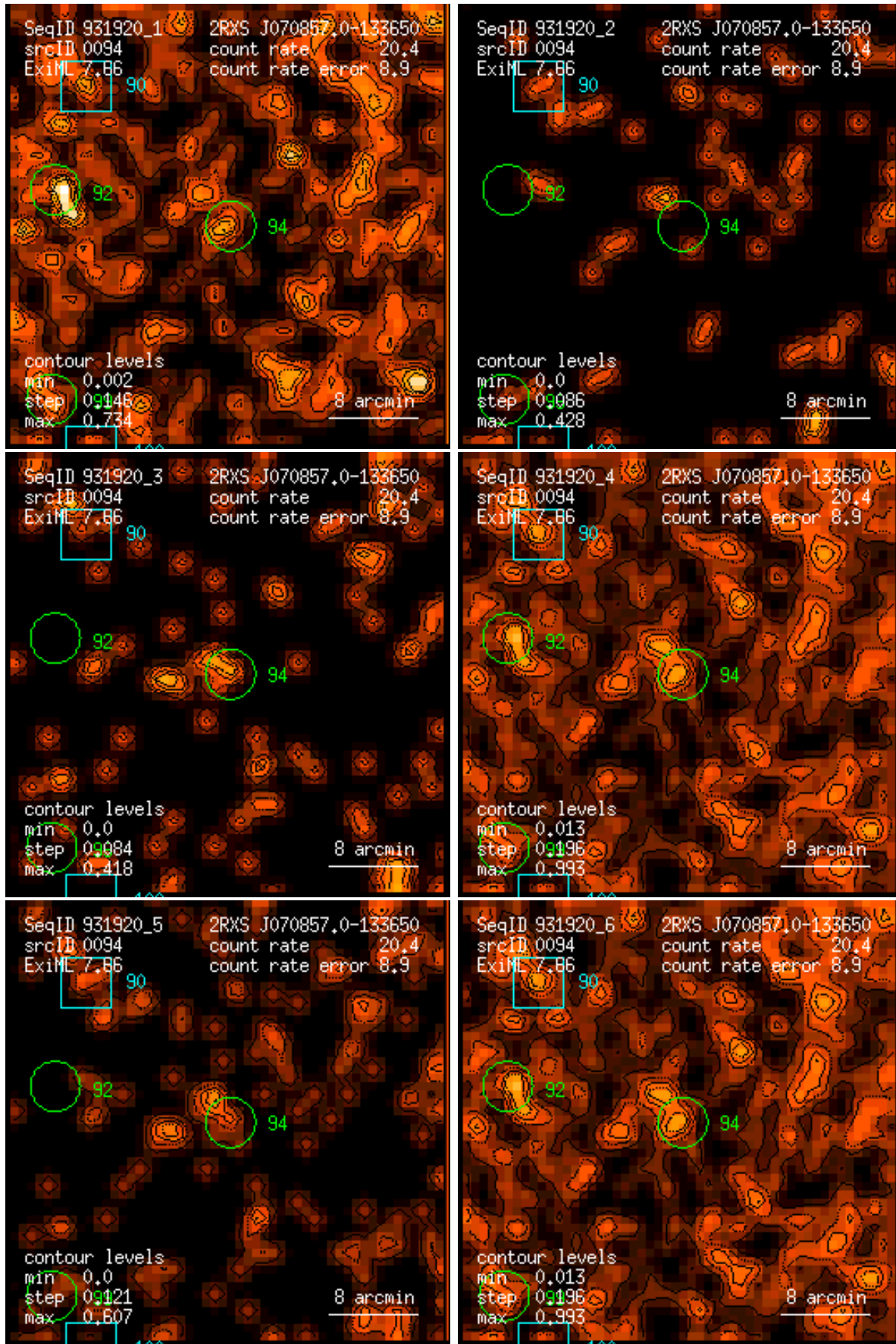
Figure 94: RASS 931920: detection 0094: band rate images, Gaussian filter: (1) PSPC channels 11 – 41, (2) 52 – 90, (3) 91 – 201, (4) 11 – 235, (5) 52 – 201, (6) 11 – 201. Broad band rates in counts/ks. Band rate contour levels in counts/ks/arcmin 2 .
