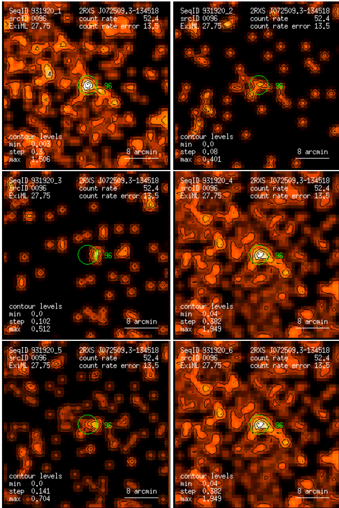
Figure 96: RASS 931920: detection 0096: band rate images, Gaussian filter: (1) PSPC channels 11 – 41, (2) 52 – 90, (3) 91 – 201, (4) 11 – 235, (5) 52 – 201, (6) 11 – 201. Broad band rates in counts/ks. Band rate contour levels in counts/ks/arcmin 2 .
