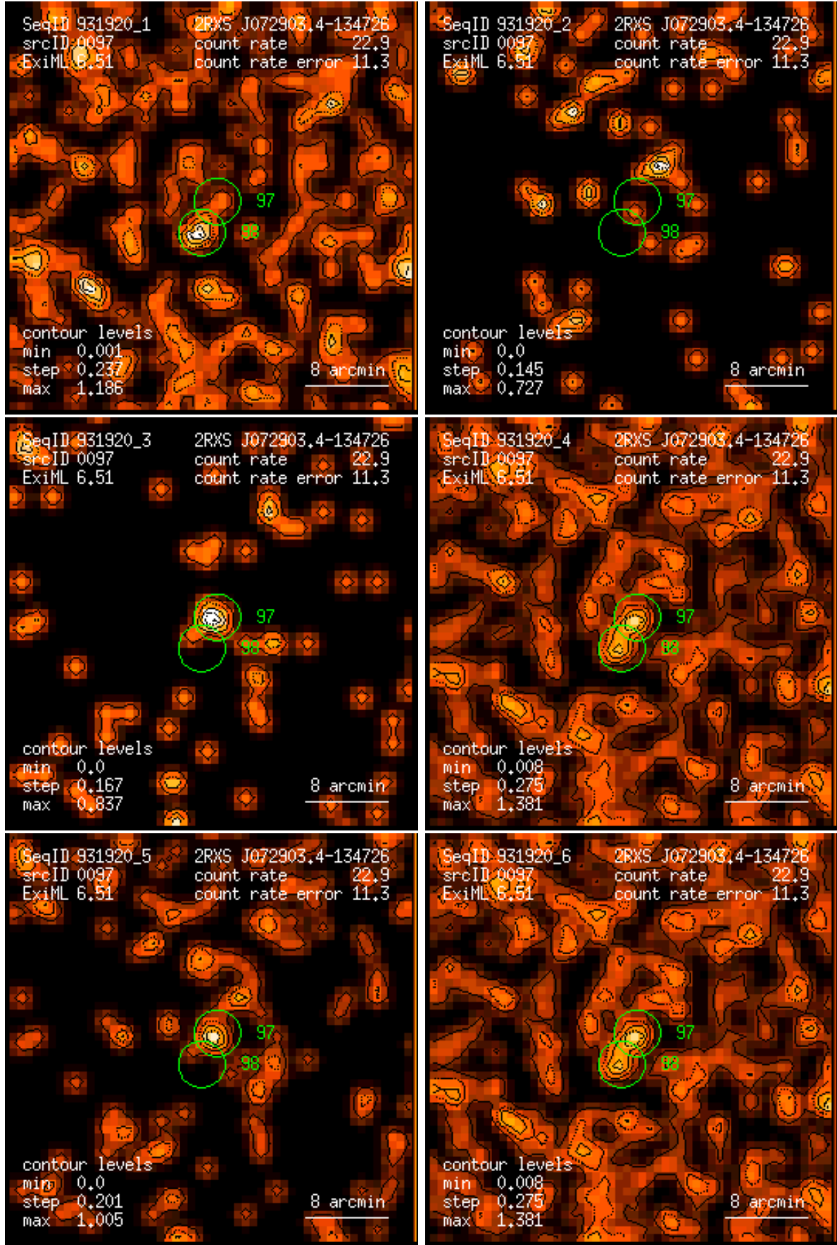
Figure 97: RASS 931920: detection 0097: band rate images, Gaussian filter: (1) PSPC channels 11 – 41, (2) 52 – 90, (3) 91 – 201, (4) 11 – 235, (5) 52 – 201, (6) 11 – 201. Broad band rates in counts/ks. Band rate contour levels in counts/ks/arcmin 2 .
