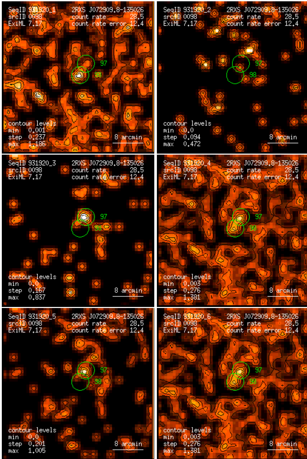
Figure 98: RASS 931920: detection 0098: band rate images, Gaussian filter: (1) PSPC channels 11 – 41, (2) 52 – 90, (3) 91 – 201, (4) 11 – 235, (5) 52 – 201, (6) 11 – 201. Broad band rates in counts/ks. Band rate contour levels in counts/ks/arcmin 2 .
