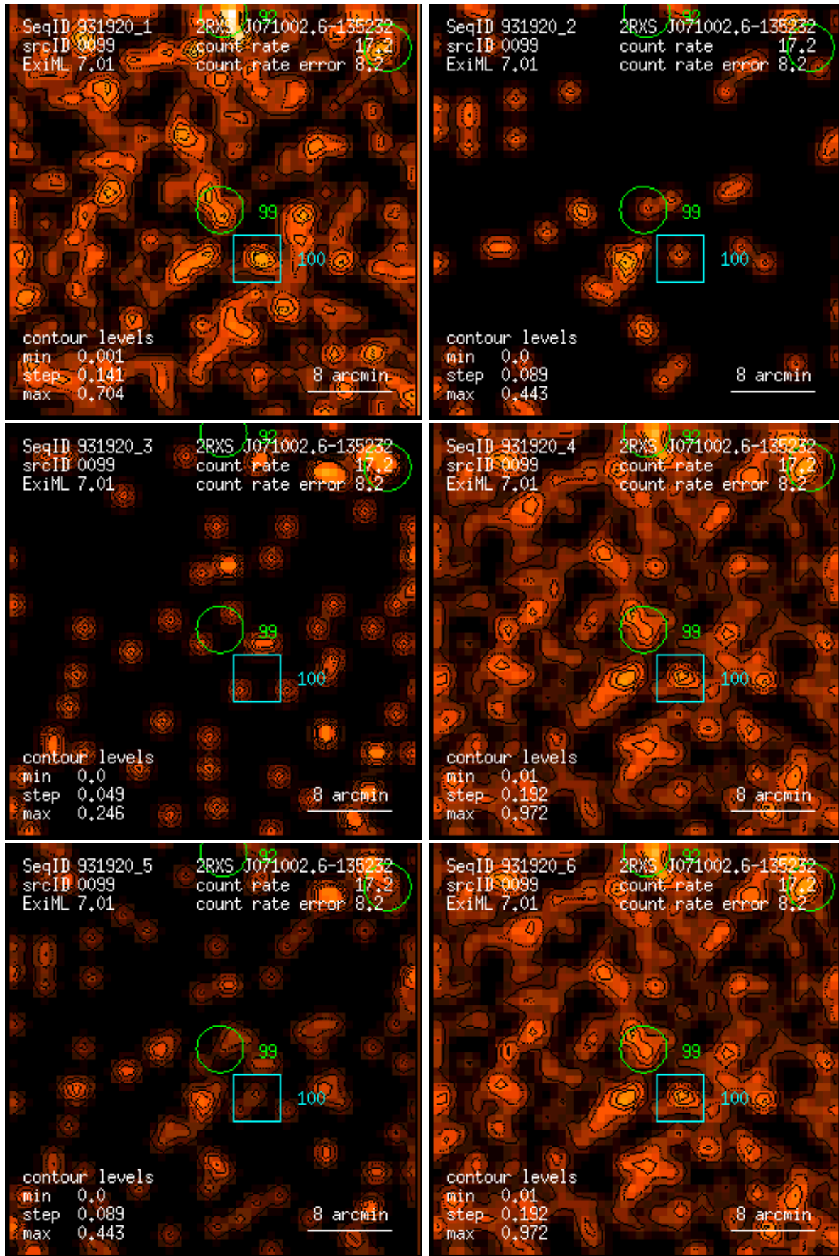
Figure 99: RASS 931920: detection 0099: band rate images, Gaussian filter: (1) PSPC channels 11 – 41, (2) 52 – 90, (3) 91 – 201, (4) 11 – 235, (5) 52 – 201, (6) 11 – 201. Broad band rates in counts/ks. Band rate contour levels in counts/ks/arcmin 2 .
