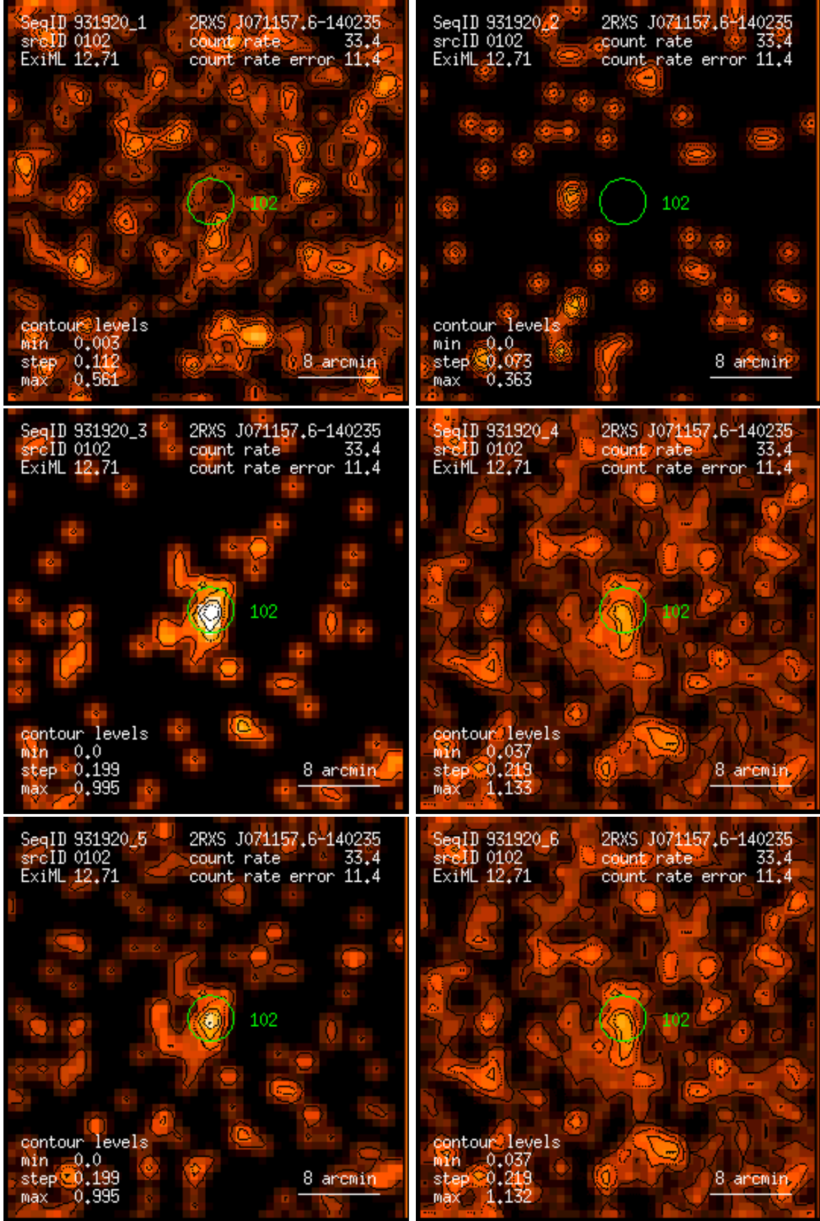
Figure 102: RASS 931920: detection 0102: band rate images, Gaussian filter: (1) PSPC channels 11 – 41, (2) 52 – 90, (3) 91 – 201, (4) 11 – 235, (5) 52 – 201, (6) 11 – 201. Broad band rates in counts/ks. Band rate contour levels in counts/ks/arcmin 2 .
