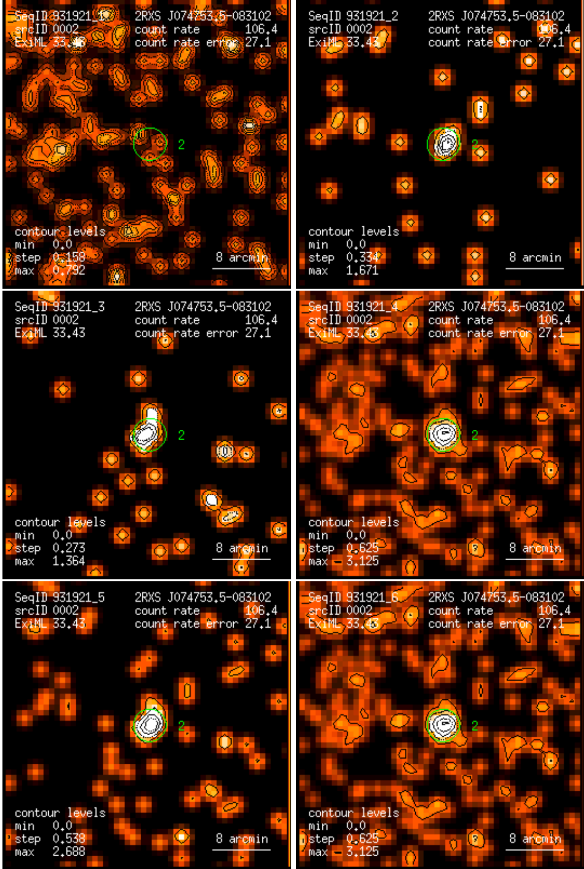
Figure 2: RASS 931921: detection 0002: band rate images, Gaussian filter: (1) PSPC channels 11 – 41, (2) 52 – 90, (3) 91 – 201, (4) 11 – 235, (5) 52 – 201, (6) 11 – 201. Broad band rates in counts/ks. Band rate contour levels in counts/ks/arcmin 2 .
