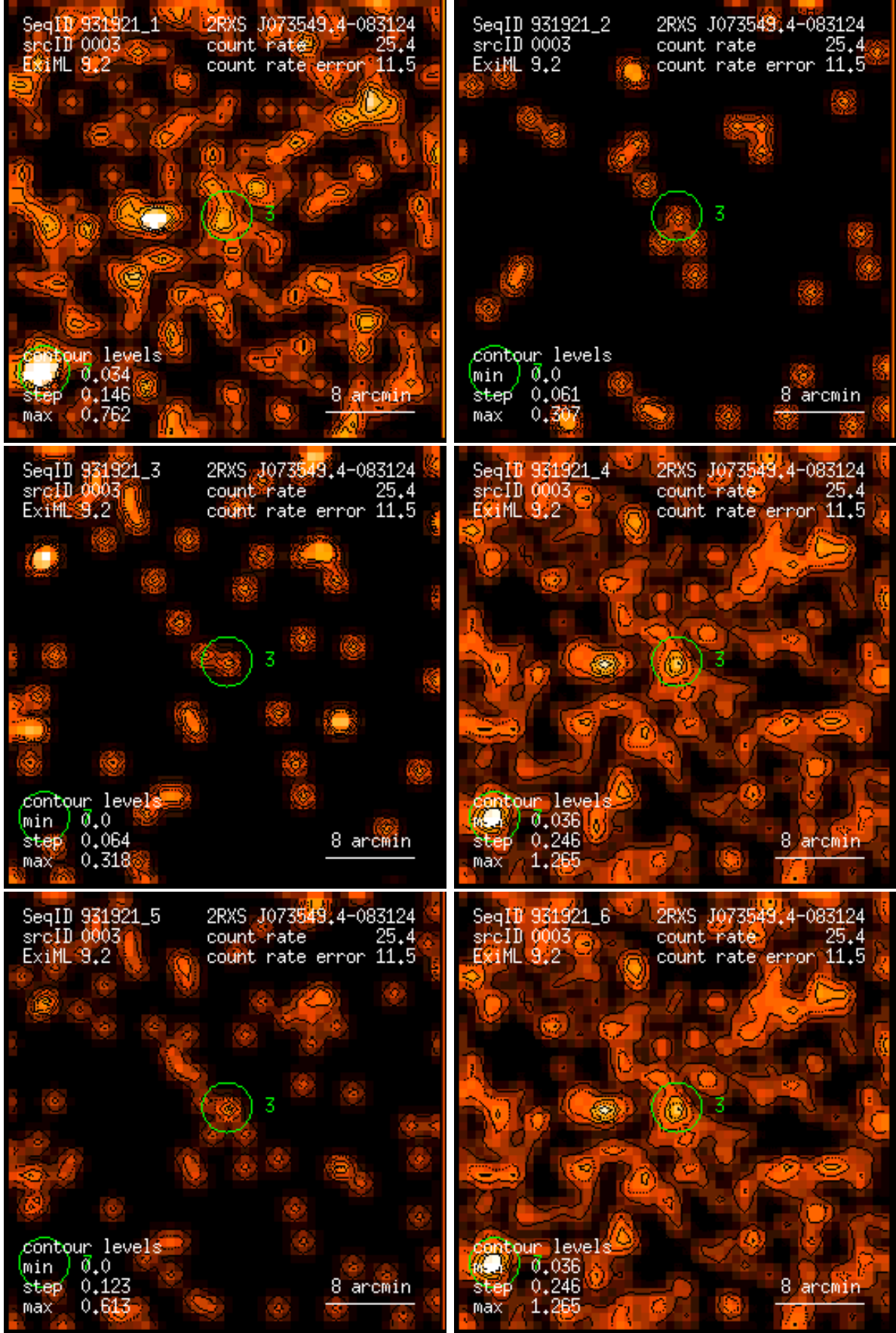
Figure 3: RASS 931921: detection 0003: band rate images, Gaussian filter: (1) PSPC channels 11 – 41, (2) 52 – 90, (3) 91 – 201, (4) 11 – 235, (5) 52 – 201, (6) 11 – 201. Broad band rates in counts/ks. Band rate contour levels in counts/ks/arcmin 2 .
