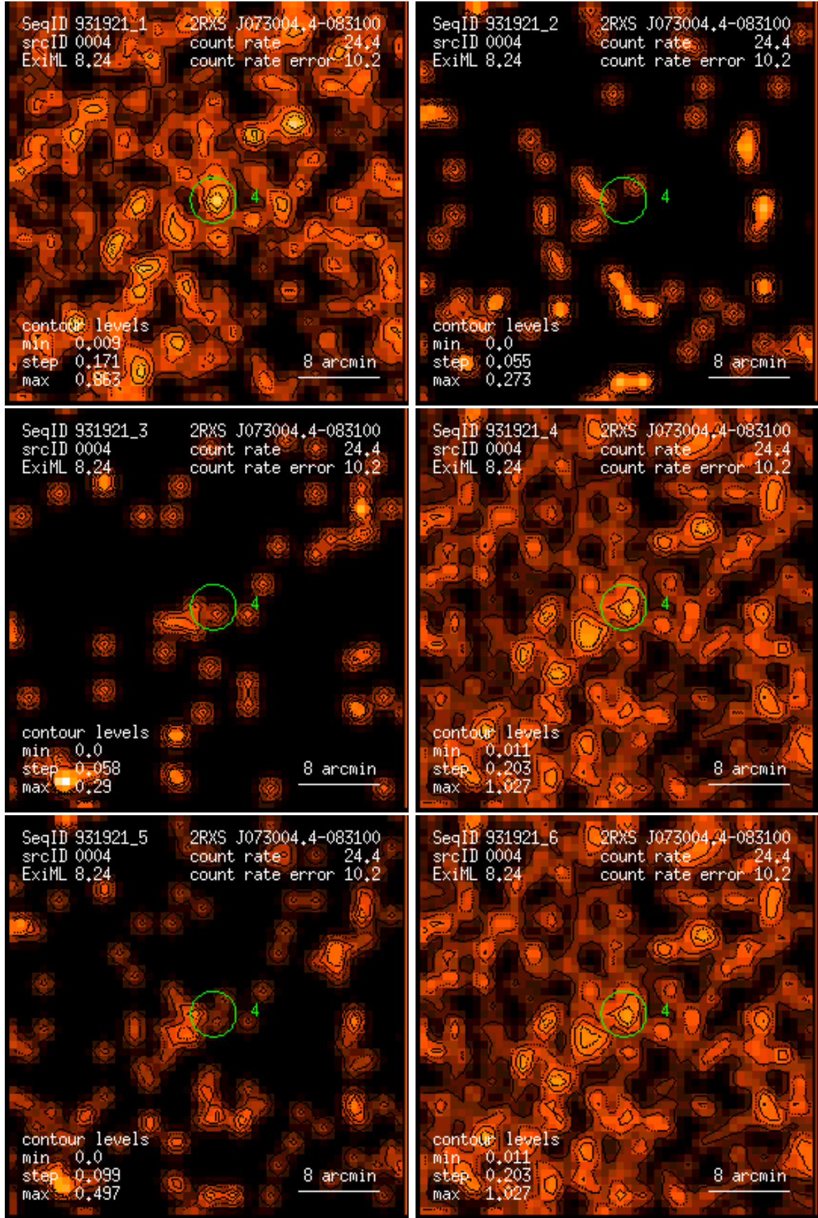
Figure 4: RASS 931921: detection 0004: band rate images, Gaussian filter: (1) PSPC channels 11 – 41, (2) 52 – 90, (3) 91 – 201, (4) 11 – 235, (5) 52 – 201, (6) 11 – 201. Broad band rates in counts/ks. Band rate contour levels in counts/ks/arcmin 2 .
