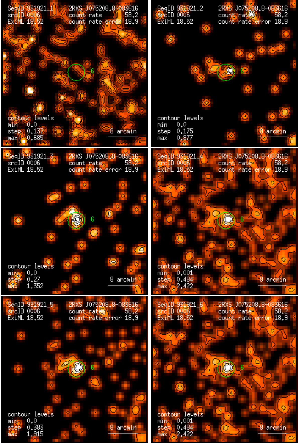
Figure 6: RASS 931921: detection 0006: band rate images, Gaussian filter: (1) PSPC channels 11 – 41, (2) 52 – 90, (3) 91 – 201, (4) 11 – 235, (5) 52 – 201, (6) 11 – 201. Broad band rates in counts/ks. Band rate contour levels in counts/ks/arcmin 2 .
