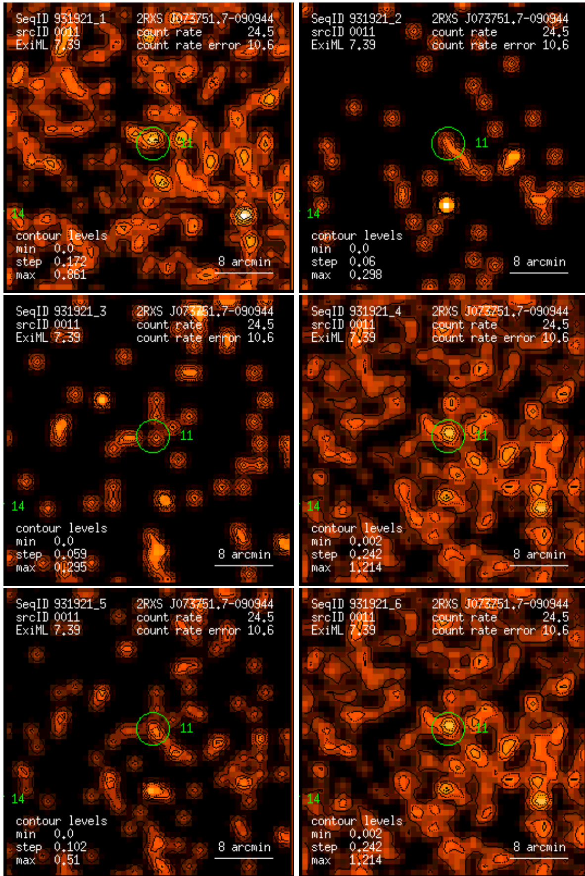
Figure 11: RASS 931921: detection 0011: band rate images, Gaussian filter: (1) PSPC channels 11 – 41, (2) 52 – 90, (3) 91 – 201, (4) 11 – 235, (5) 52 – 201, (6) 11 – 201. Broad band rates in counts/ks. Band rate contour levels in counts/ks/arcmin 2 .
