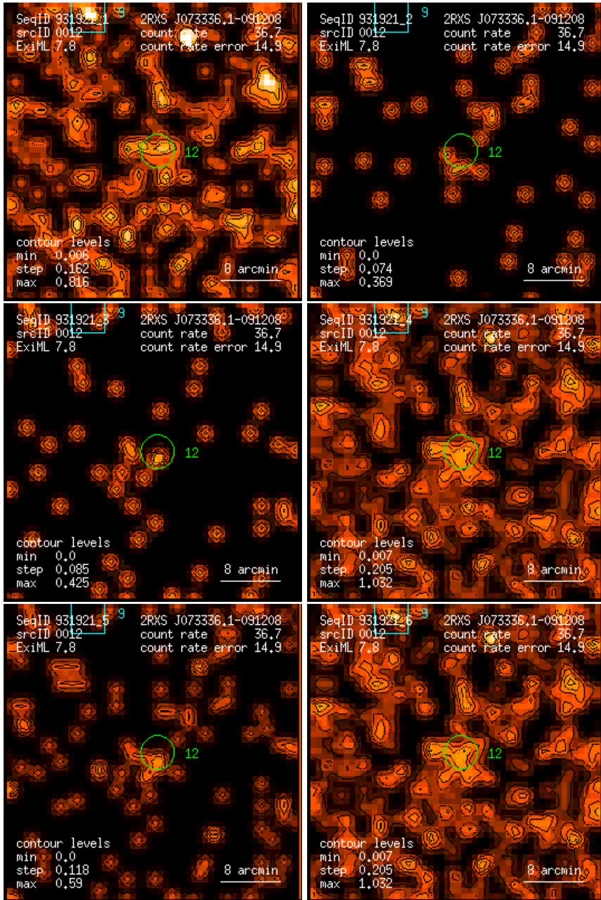
Figure 12: RASS 931921: detection 0012: band rate images, Gaussian filter: (1) PSPC channels 11 – 41, (2) 52 – 90, (3) 91 – 201, (4) 11 – 235, (5) 52 – 201, (6) 11 – 201. Broad band rates in counts/ks. Band rate contour levels in counts/ks/arcmin 2 .
