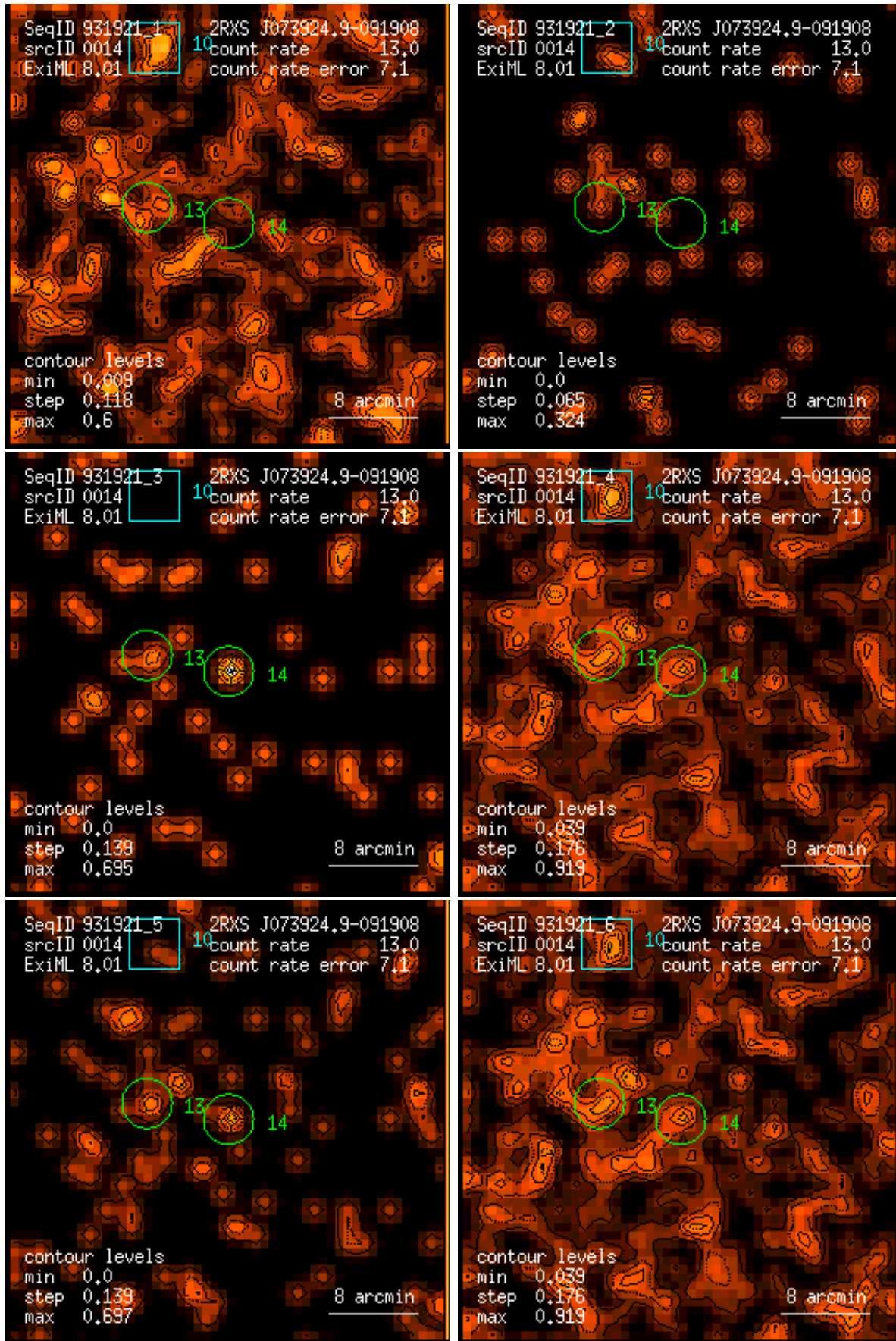
Figure 14: RASS 931921: detection 0014: band rate images, Gaussian filter: (1) PSPC channels 11 – 41, (2) 52 – 90, (3) 91 – 201, (4) 11 – 235, (5) 52 – 201, (6) 11 – 201. Broad band rates in counts/ks. Band rate contour levels in counts/ks/arcmin 2 .
