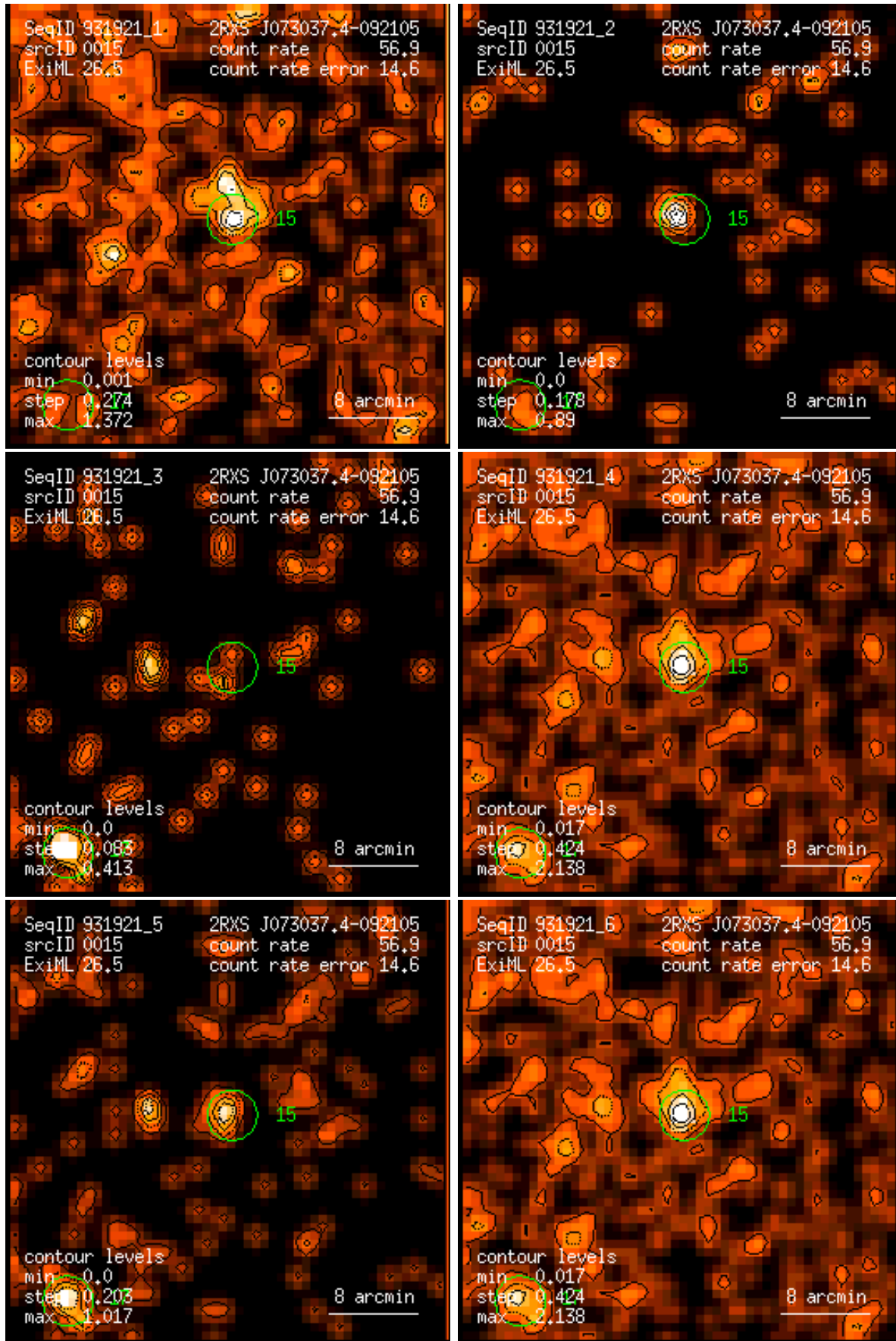
Figure 15: RASS 931921: detection 0015: band rate images, Gaussian filter: (1) PSPC channels 11 – 41, (2) 52 – 90, (3) 91 – 201, (4) 11 – 235, (5) 52 – 201, (6) 11 – 201. Broad band rates in counts/ks. Band rate contour levels in counts/ks/arcmin 2 .
