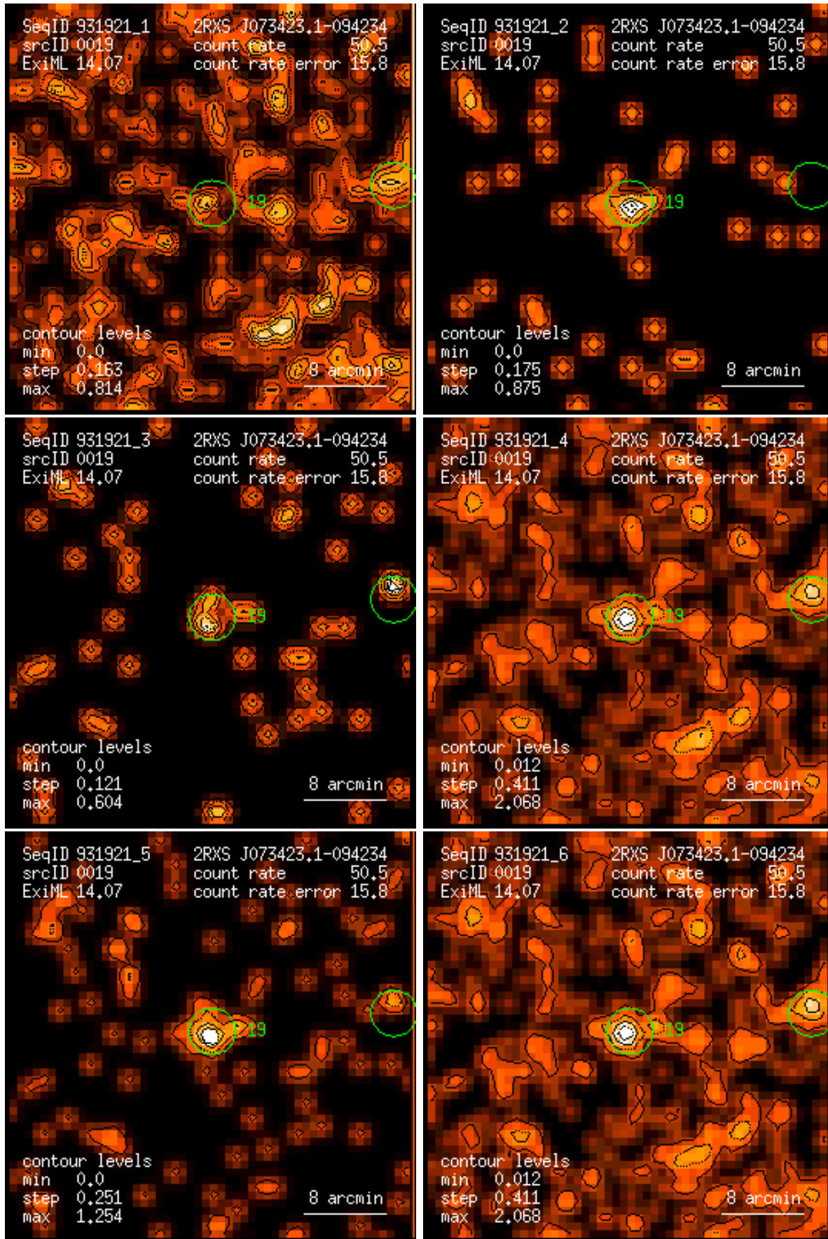
Figure 19: RASS 931921: detection 0019: band rate images, Gaussian filter: (1) PSPC channels 11 – 41, (2) 52 – 90, (3) 91 – 201, (4) 11 – 235, (5) 52 – 201, (6) 11 – 201. Broad band rates in counts/ks. Band rate contour levels in counts/ks/arcmin 2 .
