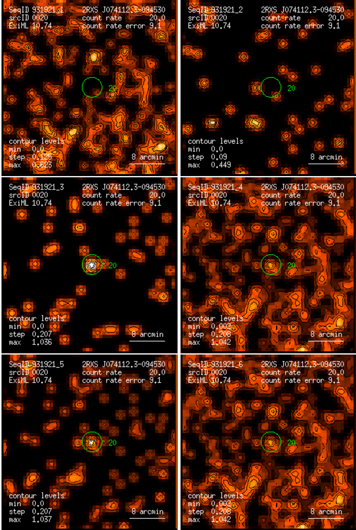
Figure 20: RASS 931921: detection 0020: band rate images, Gaussian filter: (1) PSPC channels 11 – 41, (2) 52 – 90, (3) 91 – 201, (4) 11 – 235, (5) 52 – 201, (6) 11 – 201. Broad band rates in counts/ks. Band rate contour levels in counts/ks/arcmin 2 .
