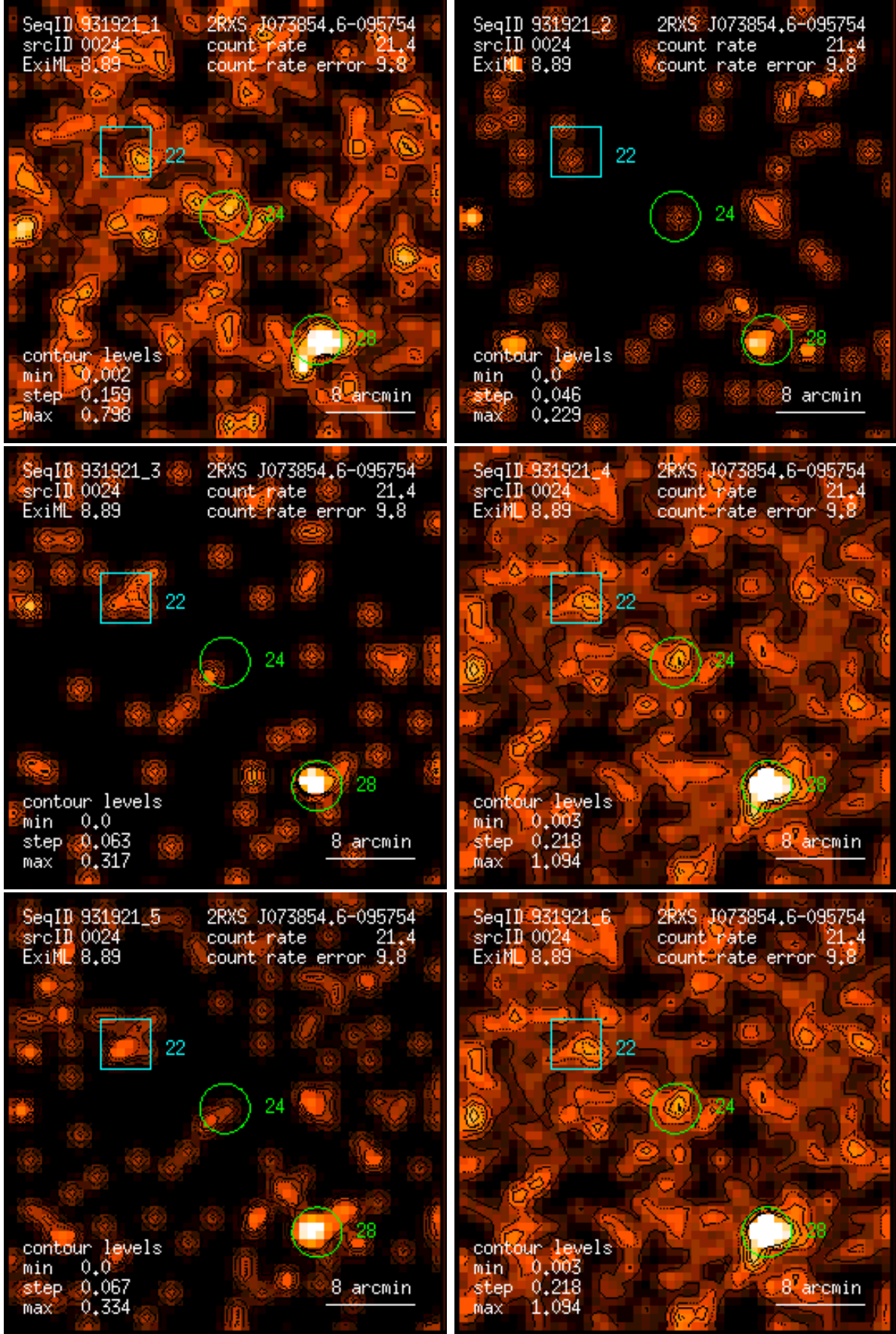
Figure 24: RASS 931921: detection 0024: band rate images, Gaussian filter: (1) PSPC channels 11 – 41, (2) 52 – 90, (3) 91 – 201, (4) 11 – 235, (5) 52 – 201, (6) 11 – 201. Broad band rates in counts/ks. Band rate contour levels in counts/ks/arcmin 2 .
