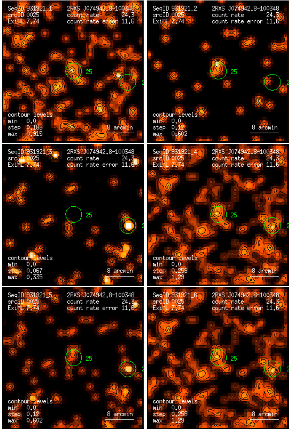
Figure 25: RASS 931921: detection 0025: band rate images, Gaussian filter: (1) PSPC channels 11 – 41, (2) 52 – 90, (3) 91 – 201, (4) 11 – 235, (5) 52 – 201, (6) 11 – 201. Broad band rates in counts/ks. Band rate contour levels in counts/ks/arcmin 2 .
