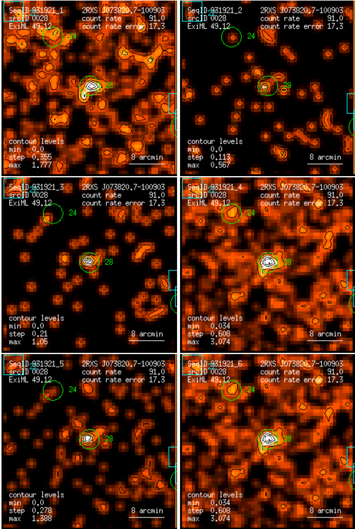
Figure 28: RASS 931921: detection 0028: band rate images, Gaussian filter: (1) PSPC channels 11 – 41, (2) 52 – 90, (3) 91 – 201, (4) 11 – 235, (5) 52 – 201, (6) 11 – 201. Broad band rates in counts/ks. Band rate contour levels in counts/ks/arcmin 2 .
