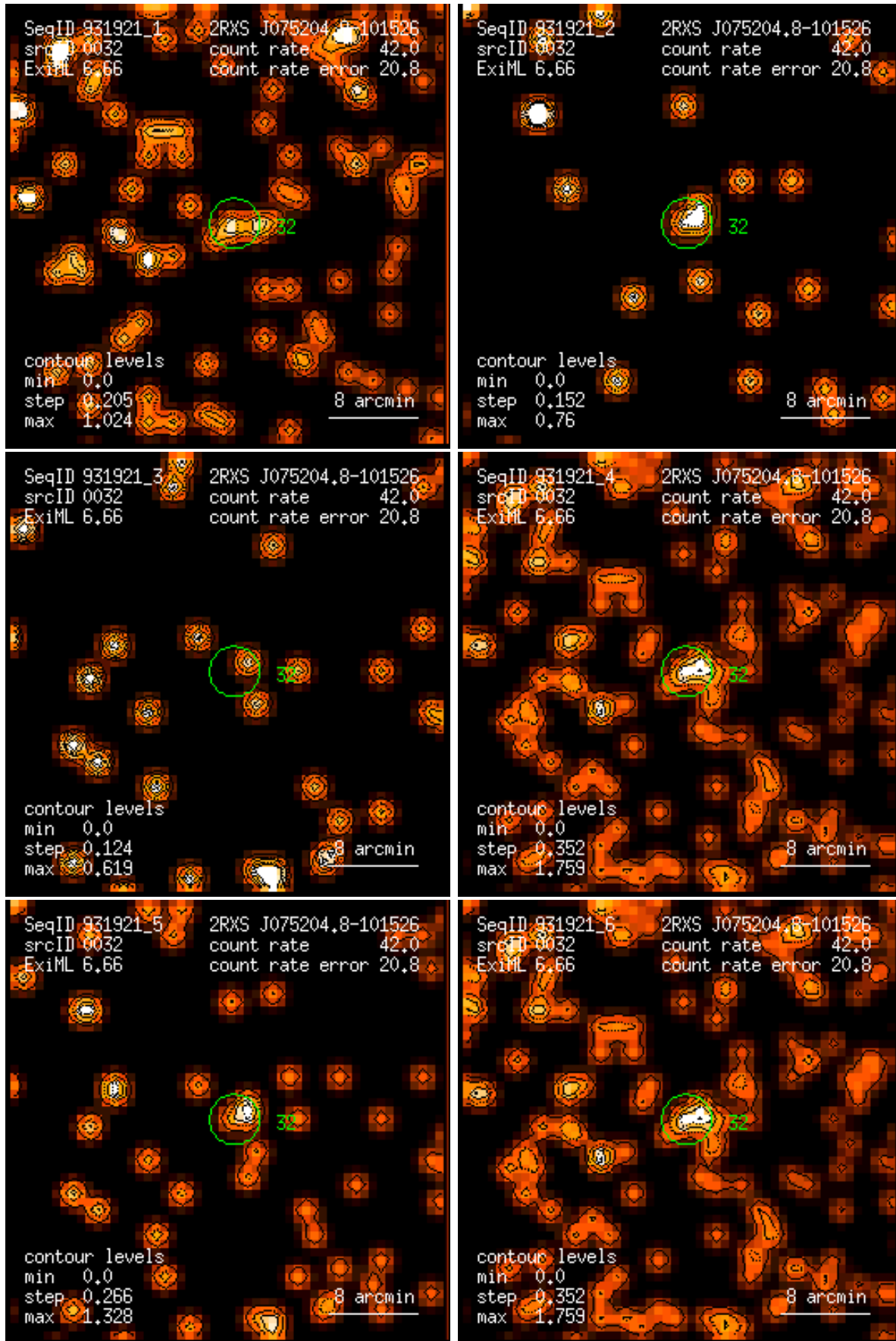
Figure 32: RASS 931921: detection 0032: band rate images, Gaussian filter: (1) PSPC channels 11 – 41, (2) 52 – 90, (3) 91 – 201, (4) 11 – 235, (5) 52 – 201, (6) 11 – 201. Broad band rates in counts/ks. Band rate contour levels in counts/ks/arcmin 2 .
