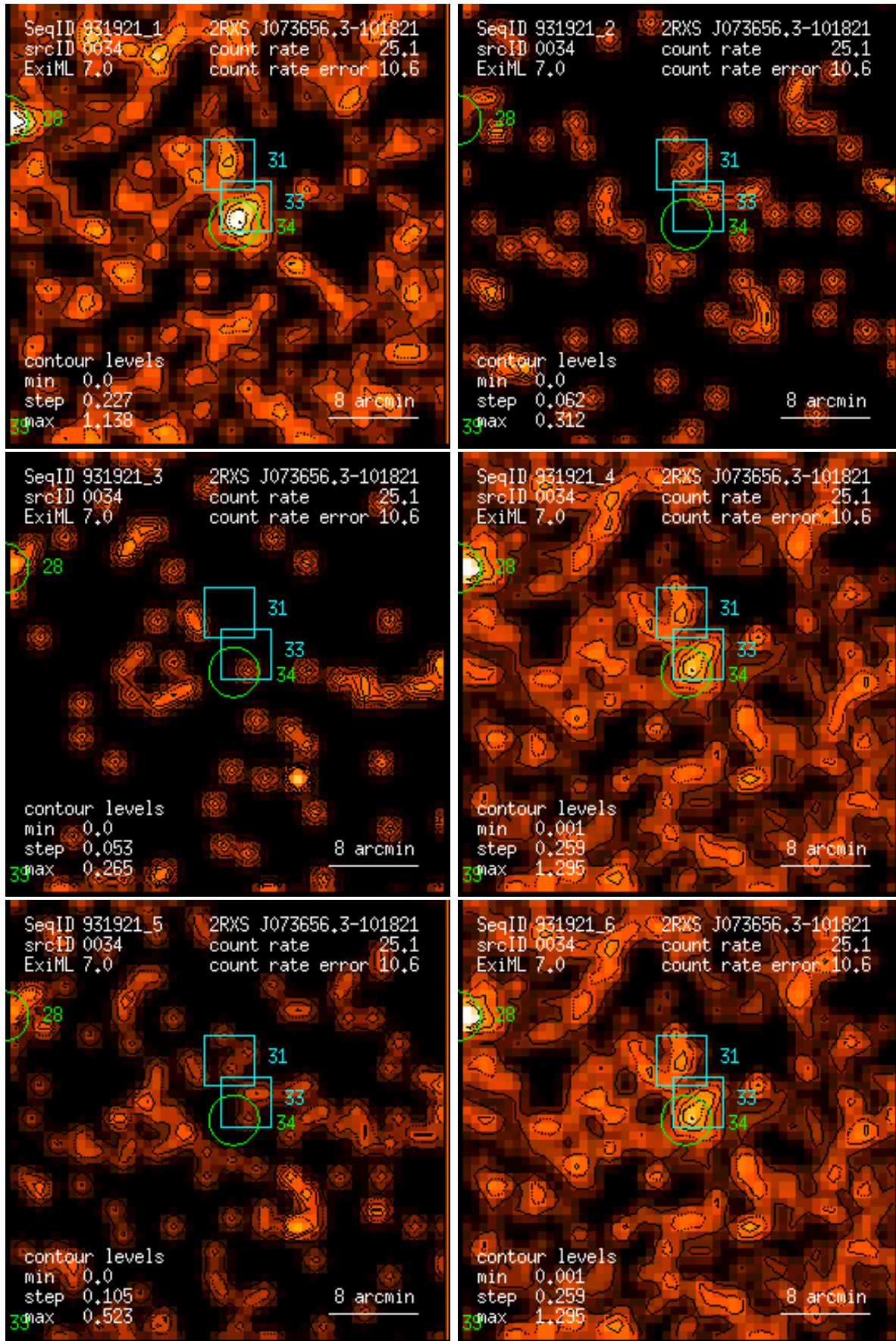
Figure 34: RASS 931921: detection 0034: band rate images, Gaussian filter: (1) PSPC channels 11 – 41, (2) 52 – 90, (3) 91 – 201, (4) 11 – 235, (5) 52 – 201, (6) 11 – 201. Broad band rates in counts/ks. Band rate contour levels in counts/ks/arcmin 2 .
