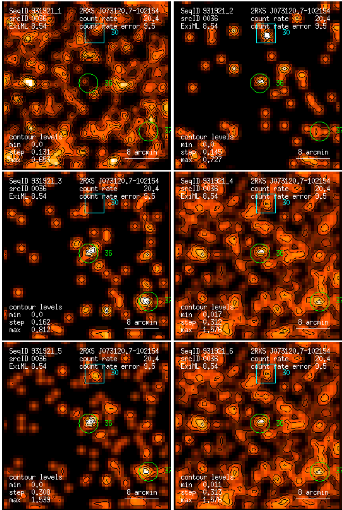
Figure 36: RASS 931921: detection 0036: band rate images, Gaussian filter: (1) PSPC channels 11 – 41, (2) 52 – 90, (3) 91 – 201, (4) 11 – 235, (5) 52 – 201, (6) 11 – 201. Broad band rates in counts/ks. Band rate contour levels in counts/ks/arcmin 2 .
