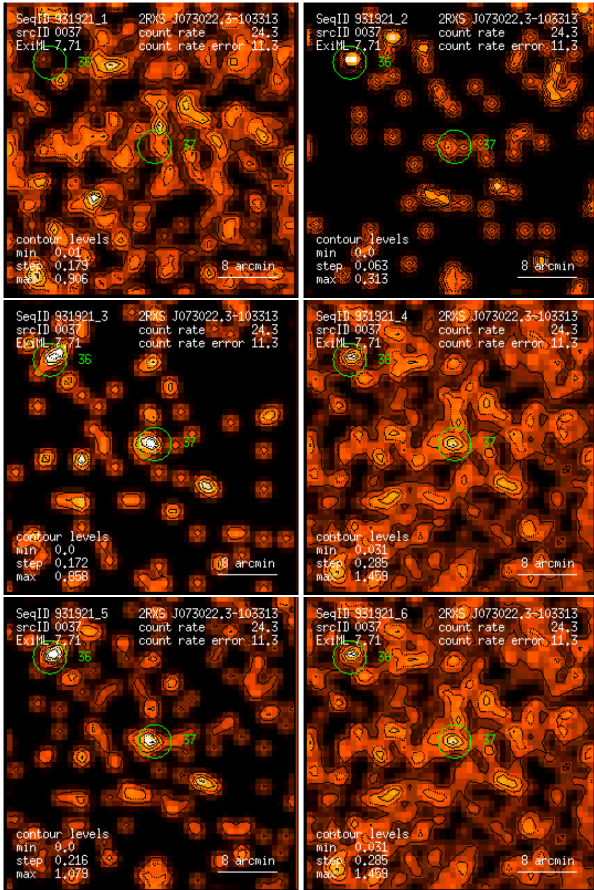
Figure 37: RASS 931921: detection 0037: band rate images, Gaussian filter: (1) PSPC channels 11 – 41, (2) 52 – 90, (3) 91 – 201, (4) 11 – 235, (5) 52 – 201, (6) 11 – 201. Broad band rates in counts/ks. Band rate contour levels in counts/ks/arcmin 2 .
