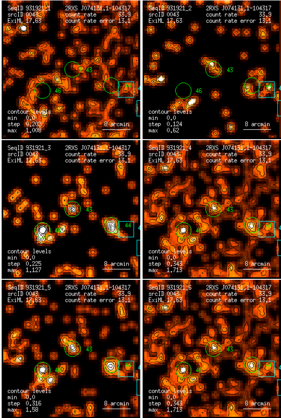
Figure 43: RASS 931921: detection 0043: band rate images, Gaussian filter: (1) PSPC channels 11 – 41, (2) 52 – 90, (3) 91 – 201, (4) 11 – 235, (5) 52 – 201, (6) 11 – 201. Broad band rates in counts/ks. Band rate contour levels in counts/ks/arcmin 2 .
