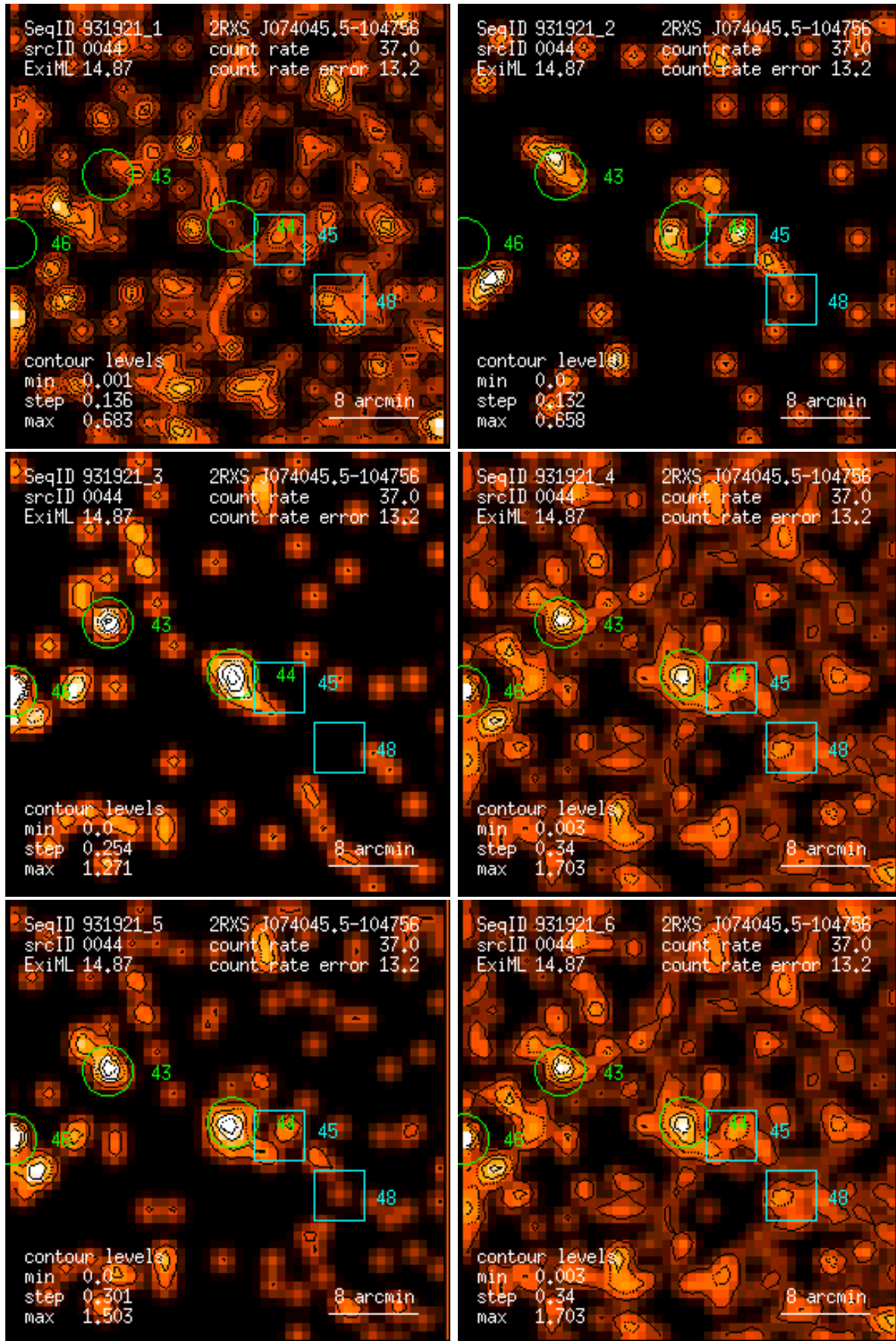
Figure 44: RASS 931921: detection 0044: band rate images, Gaussian filter: (1) PSPC channels 11 – 41, (2) 52 – 90, (3) 91 – 201, (4) 11 – 235, (5) 52 – 201, (6) 11 – 201. Broad band rates in counts/ks. Band rate contour levels in counts/ks/arcmin 2 .
