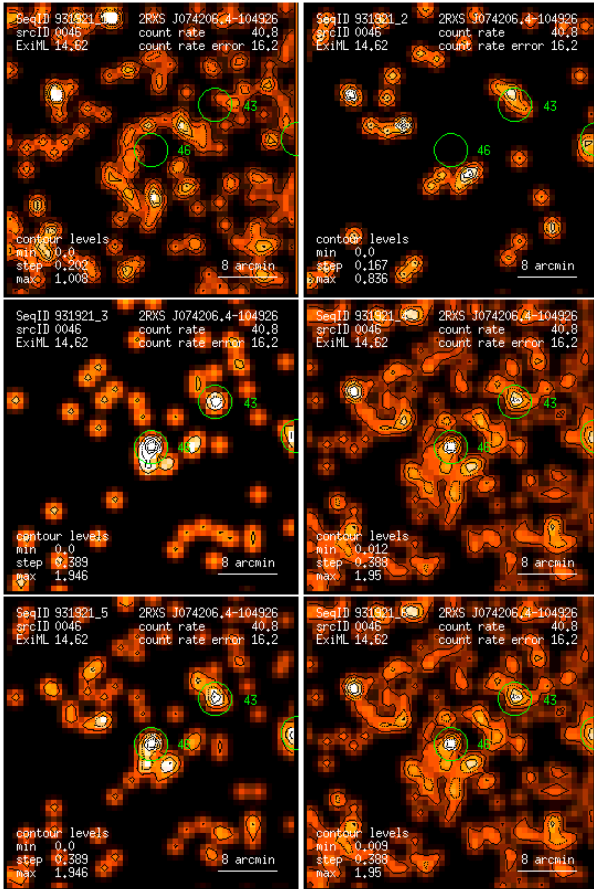
Figure 46: RASS 931921: detection 0046: band rate images, Gaussian filter: (1) PSPC channels 11 – 41, (2) 52 – 90, (3) 91 – 201, (4) 11 – 235, (5) 52 – 201, (6) 11 – 201. Broad band rates in counts/ks. Band rate contour levels in counts/ks/arcmin 2 .
