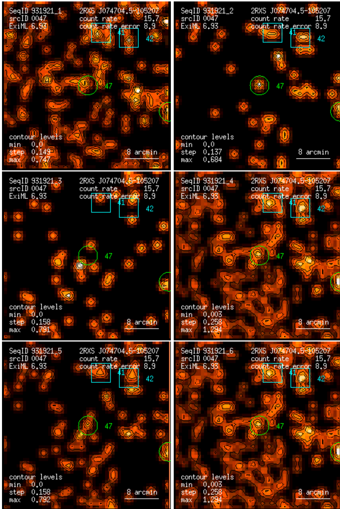
Figure 47: RASS 931921: detection 0047: band rate images, Gaussian filter: (1) PSPC channels 11 – 41, (2) 52 – 90, (3) 91 – 201, (4) 11 – 235, (5) 52 – 201, (6) 11 – 201. Broad band rates in counts/ks. Band rate contour levels in counts/ks/arcmin 2 .
