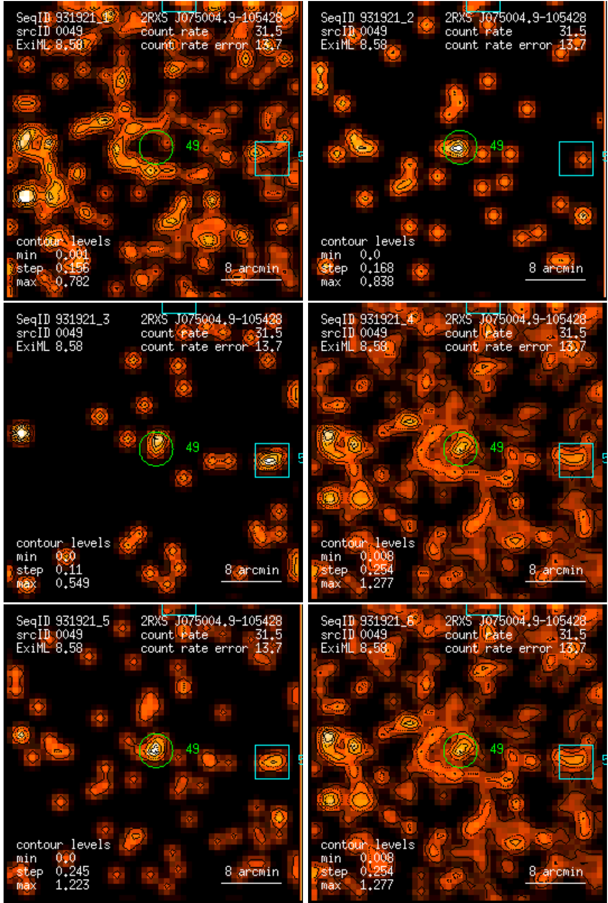
Figure 49: RASS 931921: detection 0049: band rate images, Gaussian filter: (1) PSPC channels 11 – 41, (2) 52 – 90, (3) 91 – 201, (4) 11 – 235, (5) 52 – 201, (6) 11 – 201. Broad band rates in counts/ks. Band rate contour levels in counts/ks/arcmin 2 .
