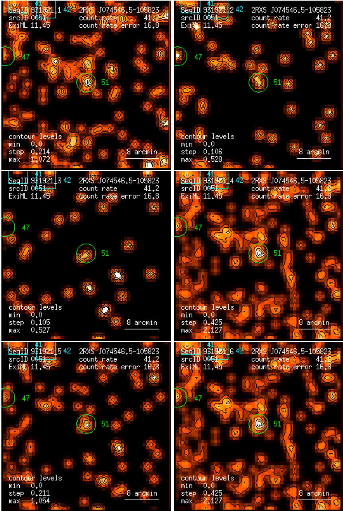
Figure 51: RASS 931921: detection 0051: band rate images, Gaussian filter: (1) PSPC channels 11 – 41, (2) 52 – 90, (3) 91 – 201, (4) 11 – 235, (5) 52 – 201, (6) 11 – 201. Broad band rates in counts/ks. Band rate contour levels in counts/ks/arcmin 2 .
