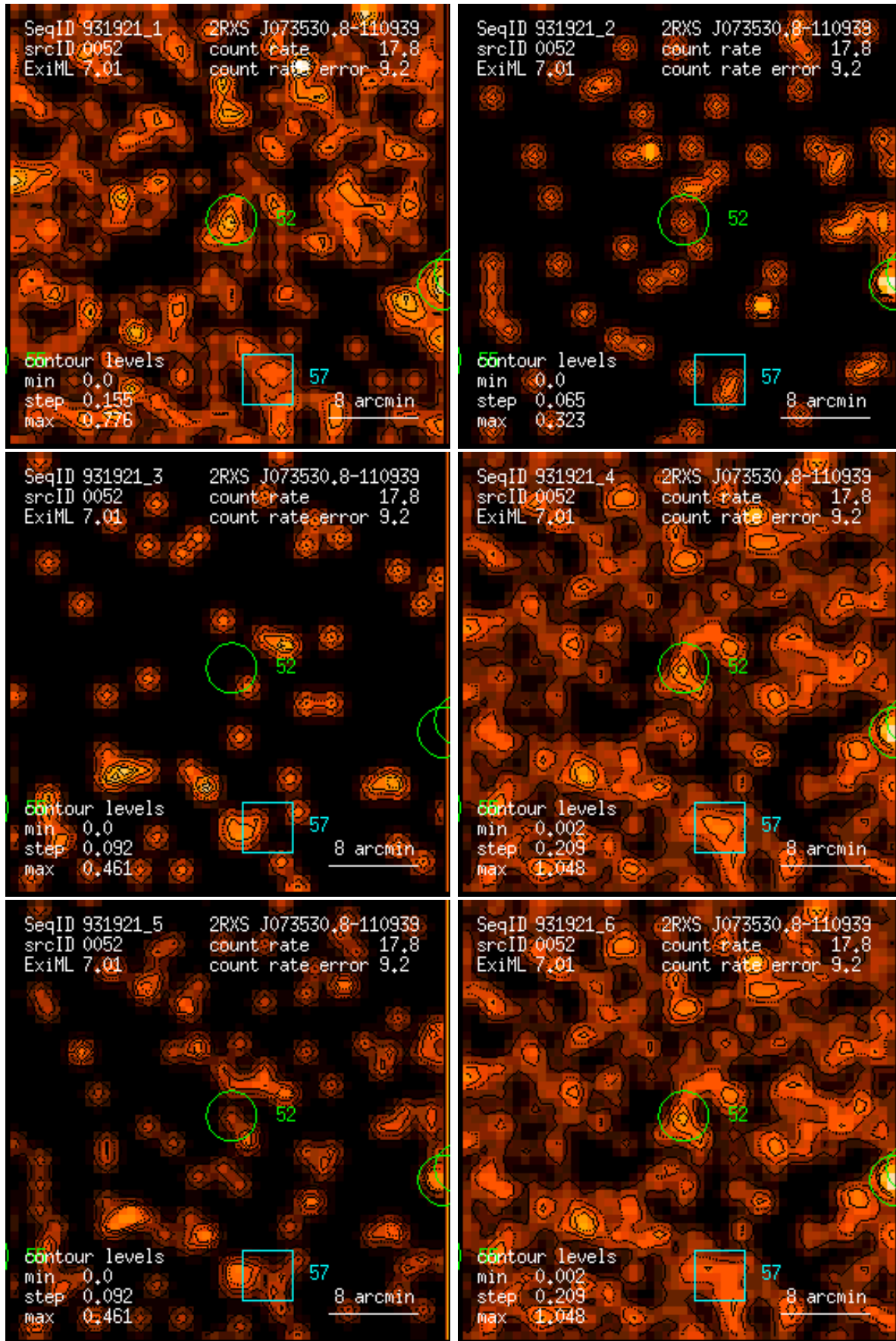
Figure 52: RASS 931921: detection 0052: band rate images, Gaussian filter: (1) PSPC channels 11 – 41, (2) 52 – 90, (3) 91 – 201, (4) 11 – 235, (5) 52 – 201, (6) 11 – 201. Broad band rates in counts/ks. Band rate contour levels in counts/ks/arcmin 2 .
