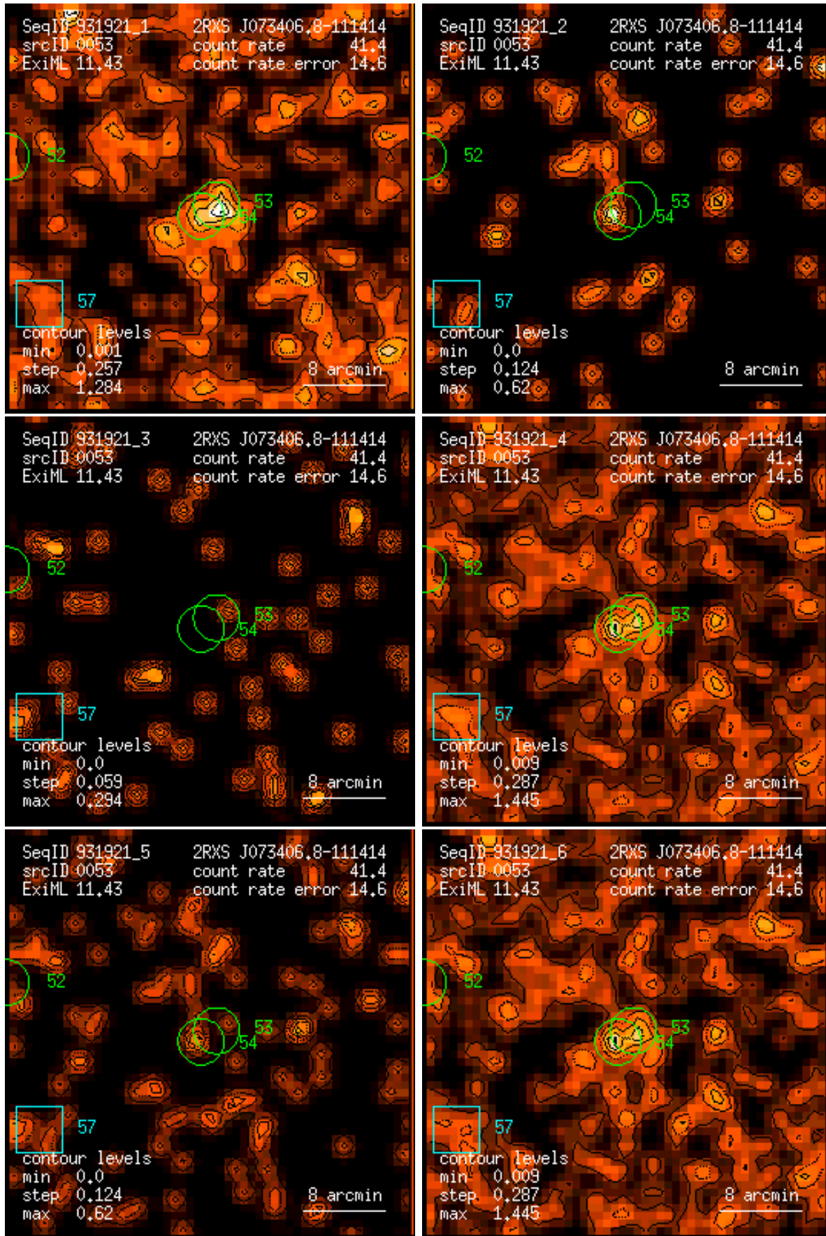
Figure 53: RASS 931921: detection 0053: band rate images, Gaussian filter: (1) PSPC channels 11 – 41, (2) 52 – 90, (3) 91 – 201, (4) 11 – 235, (5) 52 – 201, (6) 11 – 201. Broad band rates in counts/ks. Band rate contour levels in counts/ks/arcmin 2 .
