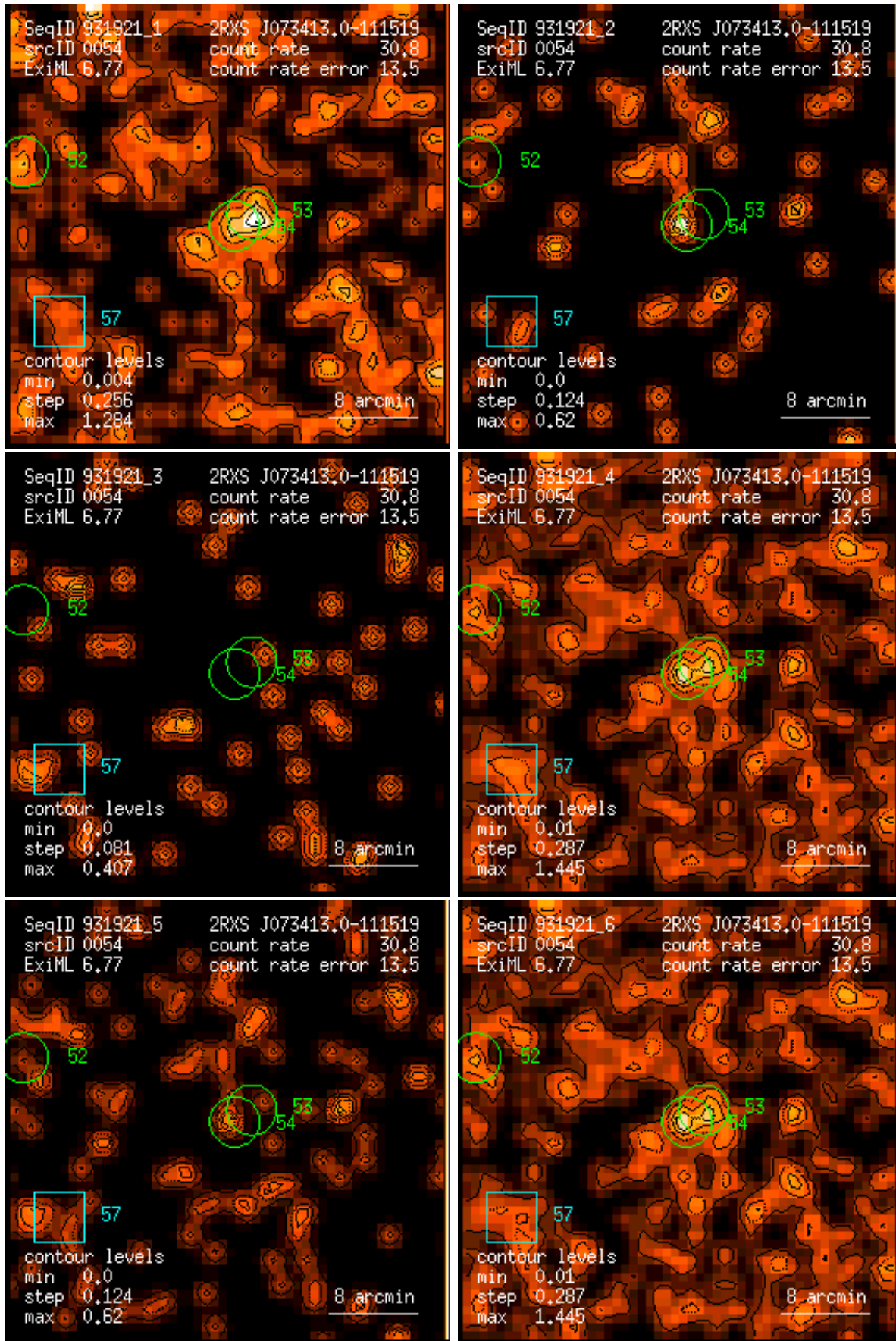
Figure 54: RASS 931921: detection 0054: band rate images, Gaussian filter: (1) PSPC channels 11 – 41, (2) 52 – 90, (3) 91 – 201, (4) 11 – 235, (5) 52 – 201, (6) 11 – 201. Broad band rates in counts/ks. Band rate contour levels in counts/ks/arcmin 2 .
