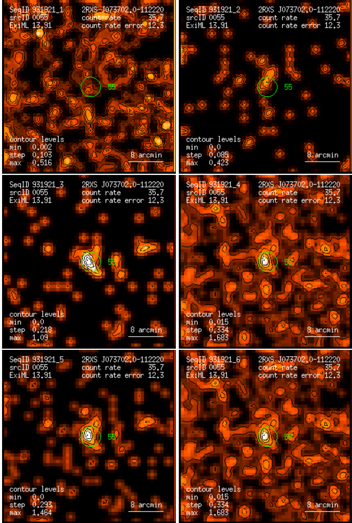
Figure 55: RASS 931921: detection 0055: band rate images, Gaussian filter: (1) PSPC channels 11 – 41, (2) 52 – 90, (3) 91 – 201, (4) 11 – 235, (5) 52 – 201, (6) 11 – 201. Broad band rates in counts/ks. Band rate contour levels in counts/ks/arcmin 2 .
