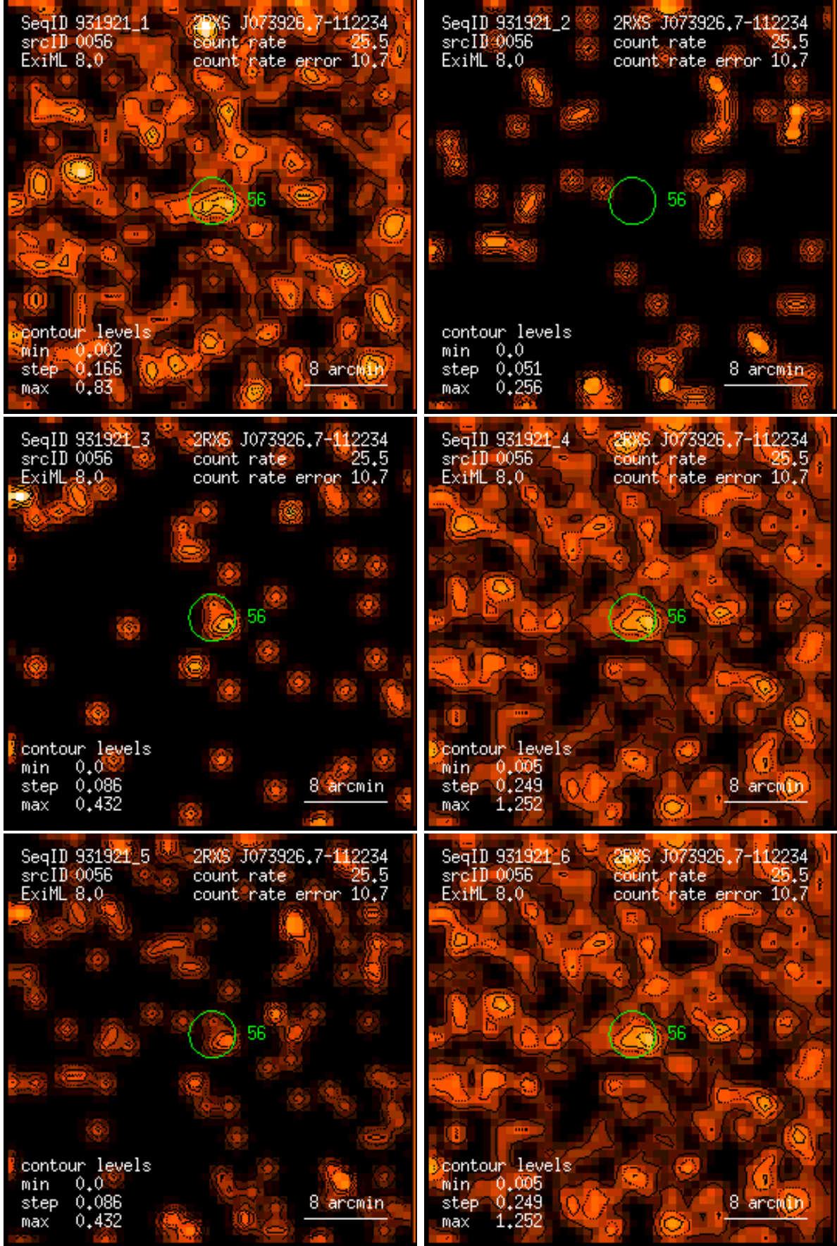
Figure 56: RASS 931921: detection 0056: band rate images, Gaussian filter: (1) PSPC channels 11 – 41, (2) 52 – 90, (3) 91 – 201, (4) 11 – 235, (5) 52 – 201, (6) 11 – 201. Broad band rates in counts/ks. Band rate contour levels in counts/ks/arcmin 2 .
