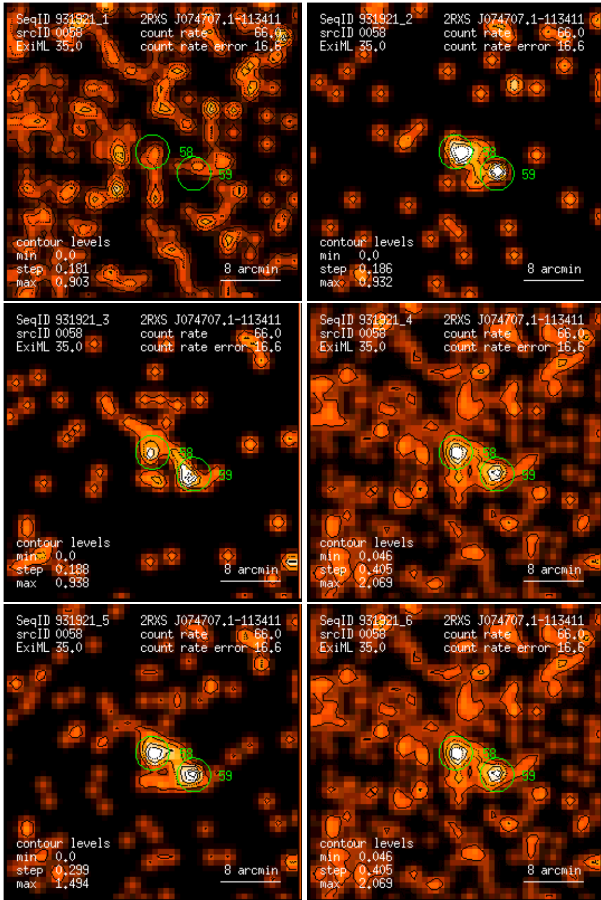
Figure 58: RASS 931921: detection 0058: band rate images, Gaussian filter: (1) PSPC channels 11 – 41, (2) 52 – 90, (3) 91 – 201, (4) 11 – 235, (5) 52 – 201, (6) 11 – 201. Broad band rates in counts/ks. Band rate contour levels in counts/ks/arcmin 2 .
