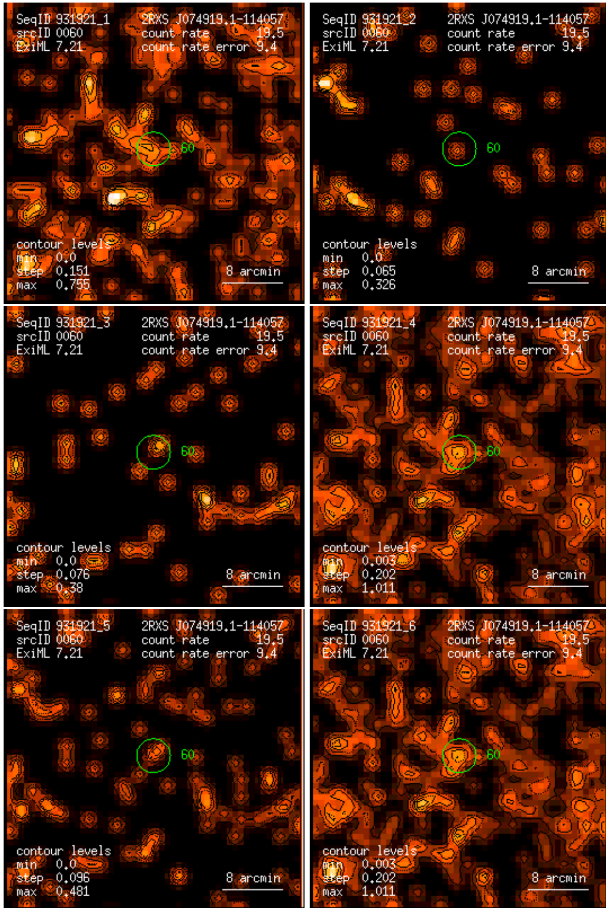
Figure 60: RASS 931921: detection 0060: band rate images, Gaussian filter: (1) PSPC channels 11 – 41, (2) 52 – 90, (3) 91 – 201, (4) 11 – 235, (5) 52 – 201, (6) 11 – 201. Broad band rates in counts/ks. Band rate contour levels in counts/ks/arcmin 2 .
