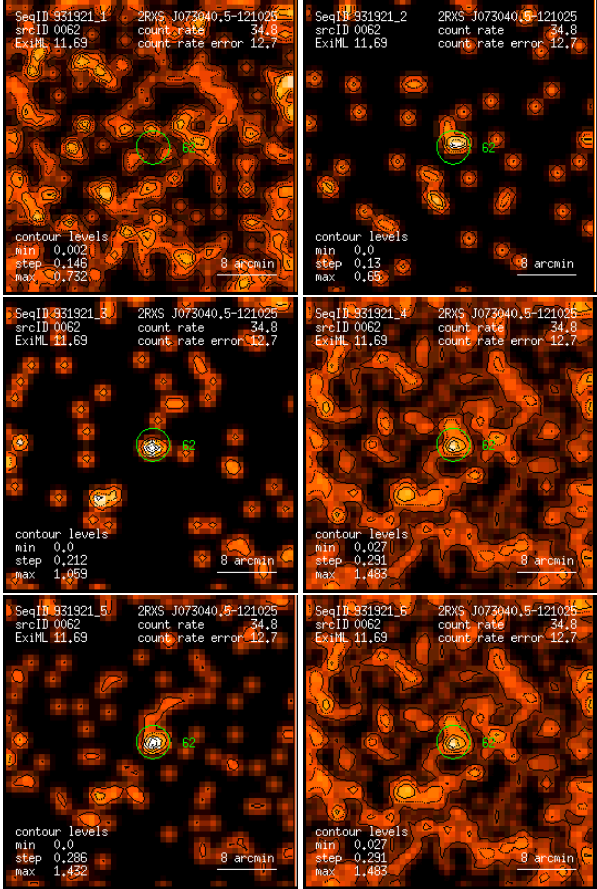
Figure 62: RASS 931921: detection 0062: band rate images, Gaussian filter: (1) PSPC channels 11 – 41, (2) 52 – 90, (3) 91 – 201, (4) 11 – 235, (5) 52 – 201, (6) 11 – 201. Broad band rates in counts/ks. Band rate contour levels in counts/ks/arcmin 2 .
