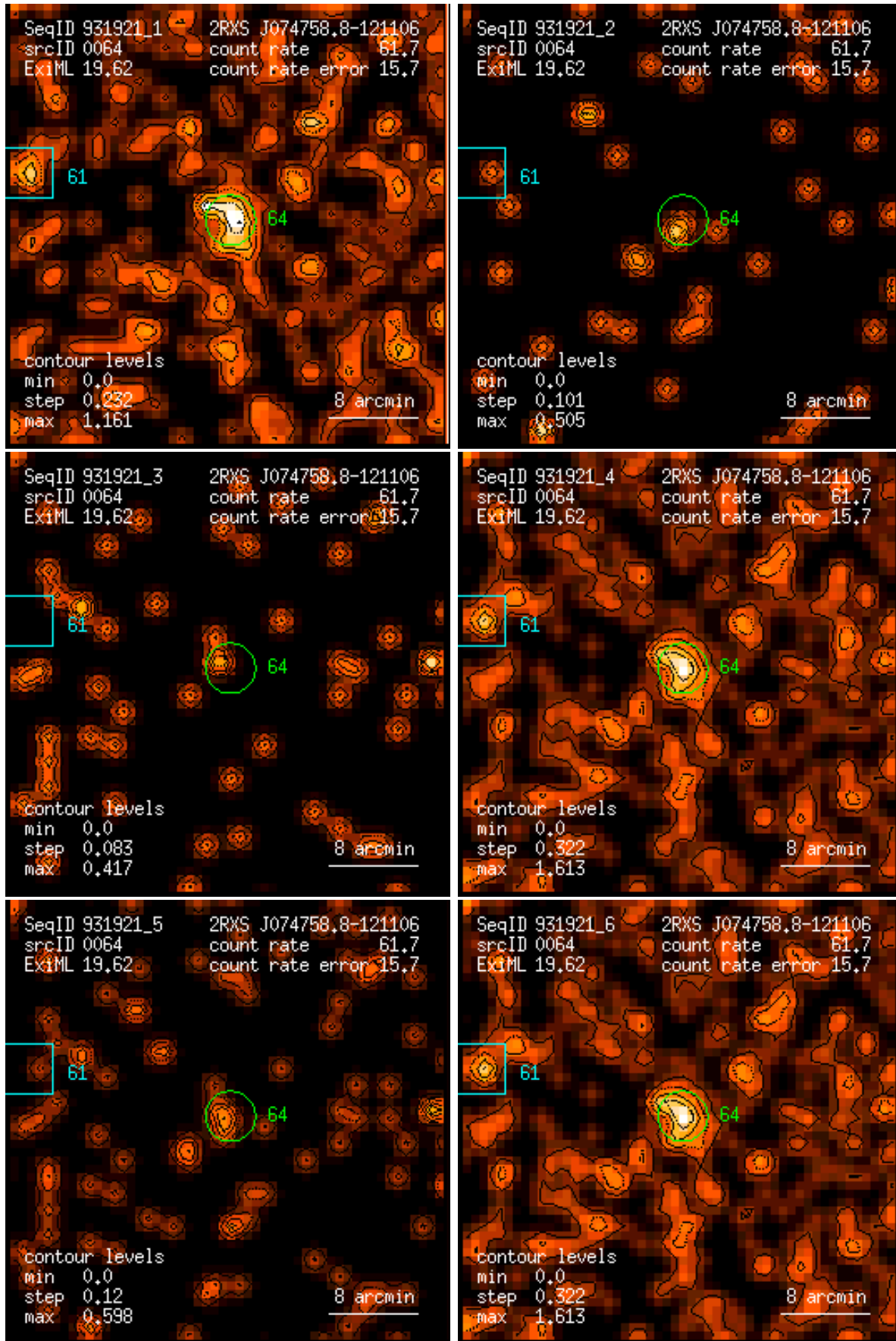
Figure 64: RASS 931921: detection 0064: band rate images, Gaussian filter: (1) PSPC channels 11 – 41, (2) 52 – 90, (3) 91 – 201, (4) 11 – 235, (5) 52 – 201, (6) 11 – 201. Broad band rates in counts/ks. Band rate contour levels in counts/ks/arcmin 2 .
