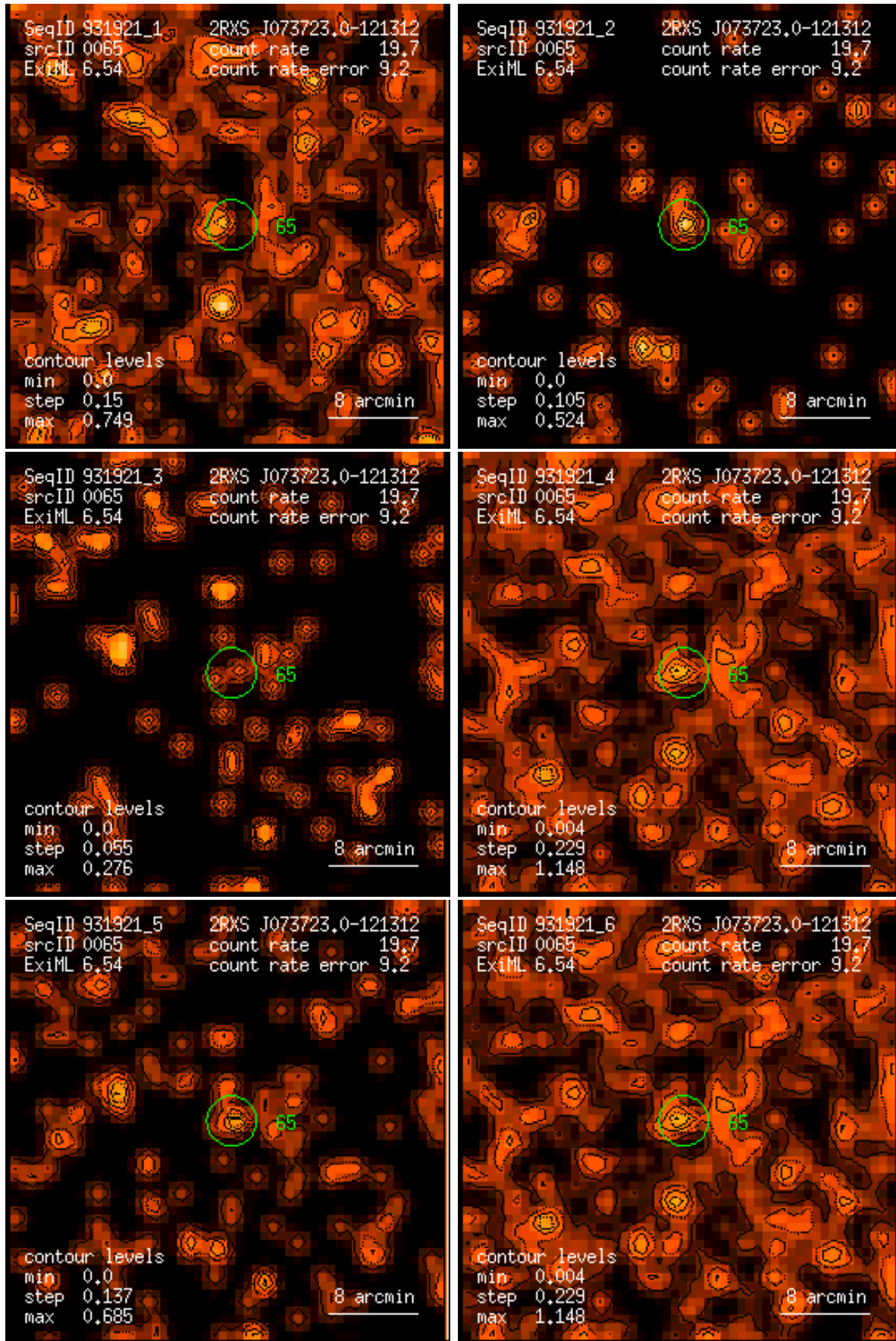
Figure 65: RASS 931921: detection 0065: band rate images, Gaussian filter: (1) PSPC channels 11 – 41, (2) 52 – 90, (3) 91 – 201, (4) 11 – 235, (5) 52 – 201, (6) 11 – 201. Broad band rates in counts/ks. Band rate contour levels in counts/ks/arcmin 2 .
