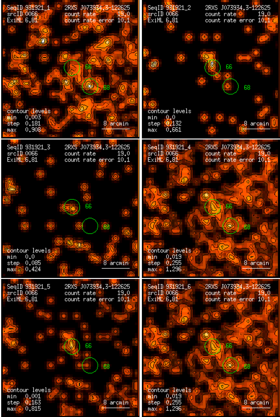
Figure 66: RASS 931921: detection 0066: band rate images, Gaussian filter: (1) PSPC channels 11 – 41, (2) 52 – 90, (3) 91 – 201, (4) 11 – 235, (5) 52 – 201, (6) 11 – 201. Broad band rates in counts/ks. Band rate contour levels in counts/ks/arcmin 2 .
