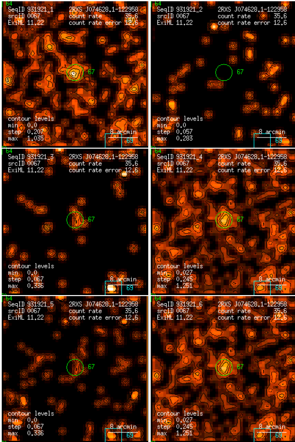
Figure 67: RASS 931921: detection 0067: band rate images, Gaussian filter: (1) PSPC channels 11 – 41, (2) 52 – 90, (3) 91 – 201, (4) 11 – 235, (5) 52 – 201, (6) 11 – 201. Broad band rates in counts/ks. Band rate contour levels in counts/ks/arcmin 2 .
