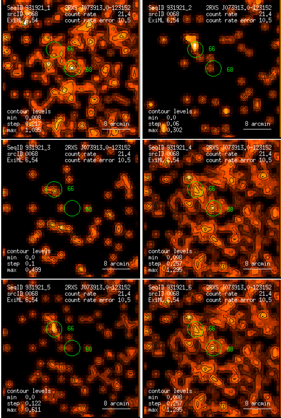
Figure 68: RASS 931921: detection 0068: band rate images, Gaussian filter: (1) PSPC channels 11 – 41, (2) 52 – 90, (3) 91 – 201, (4) 11 – 235, (5) 52 – 201, (6) 11 – 201. Broad band rates in counts/ks. Band rate contour levels in counts/ks/arcmin 2 .
