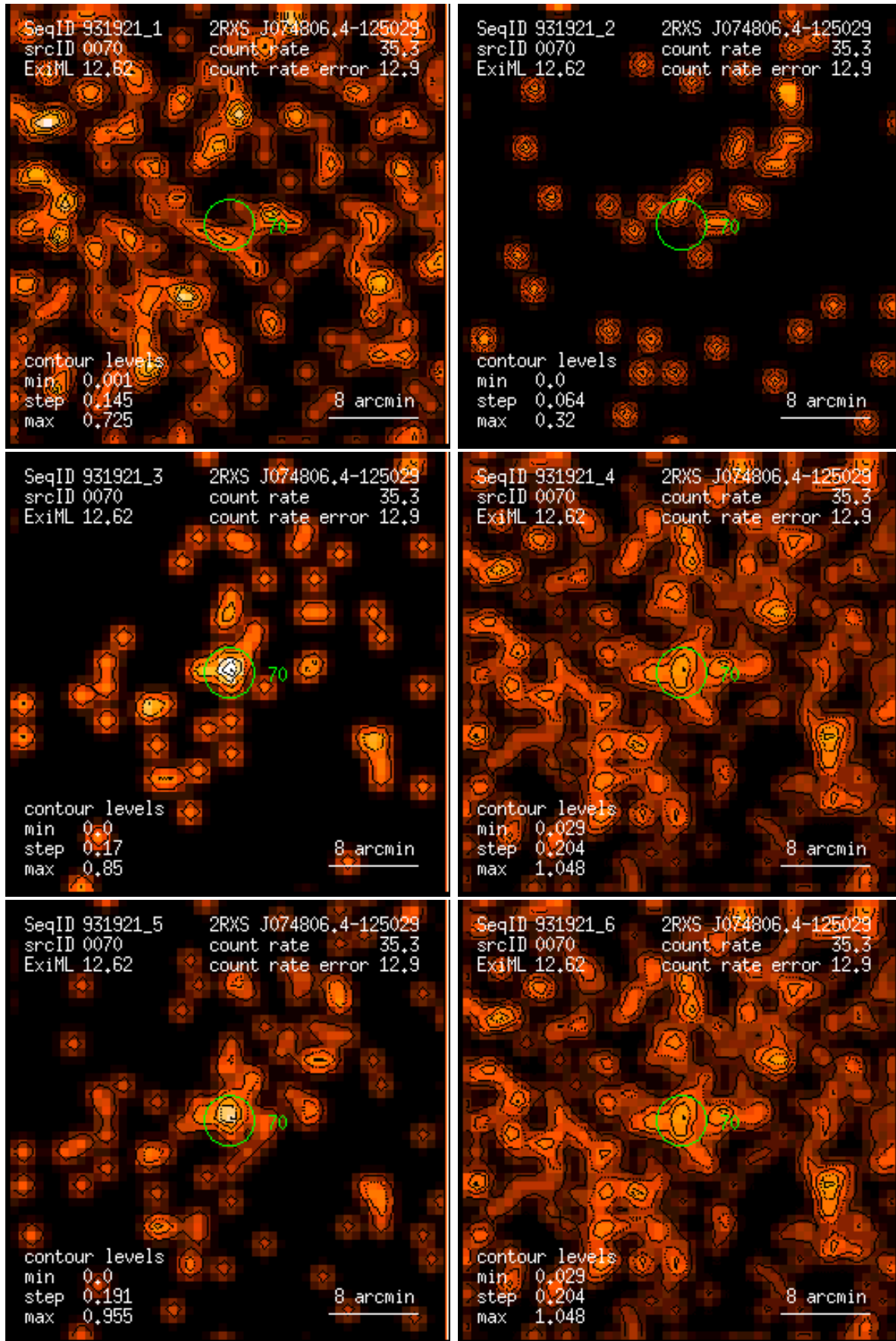
Figure 70: RASS 931921: detection 0070: band rate images, Gaussian filter: (1) PSPC channels 11 – 41, (2) 52 – 90, (3) 91 – 201, (4) 11 – 235, (5) 52 – 201, (6) 11 – 201. Broad band rates in counts/ks. Band rate contour levels in counts/ks/arcmin 2 .
